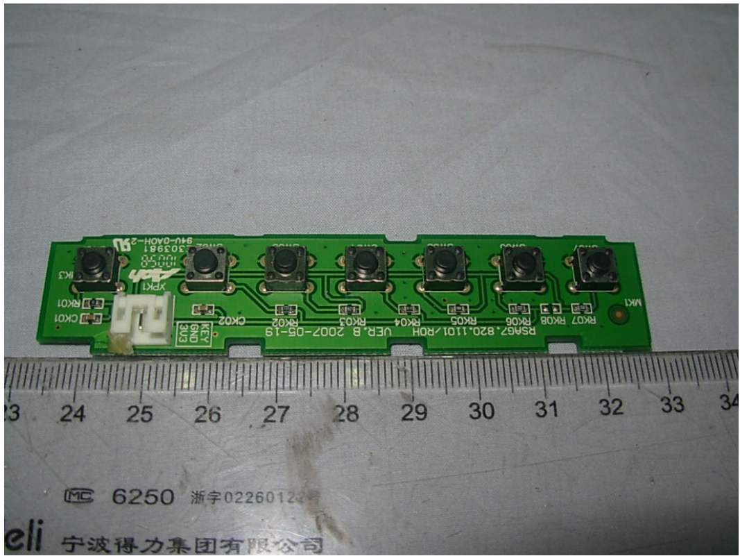
FIGURE 14 LCD TV (M/N: LTDN37W60MH) KEY BOARD (COMPONENT SIDE)
