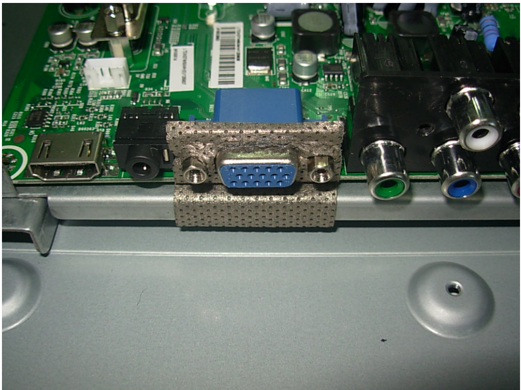
FIGURE 21 LCD TV (M/N: LTDN37W60MH) DEBUG#2
