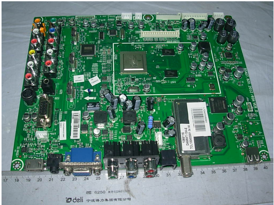
FIGURE 5 LCD TV (M/N: LTDN37W60MH) MAIN BOARD (COMPONENT SIDE)
