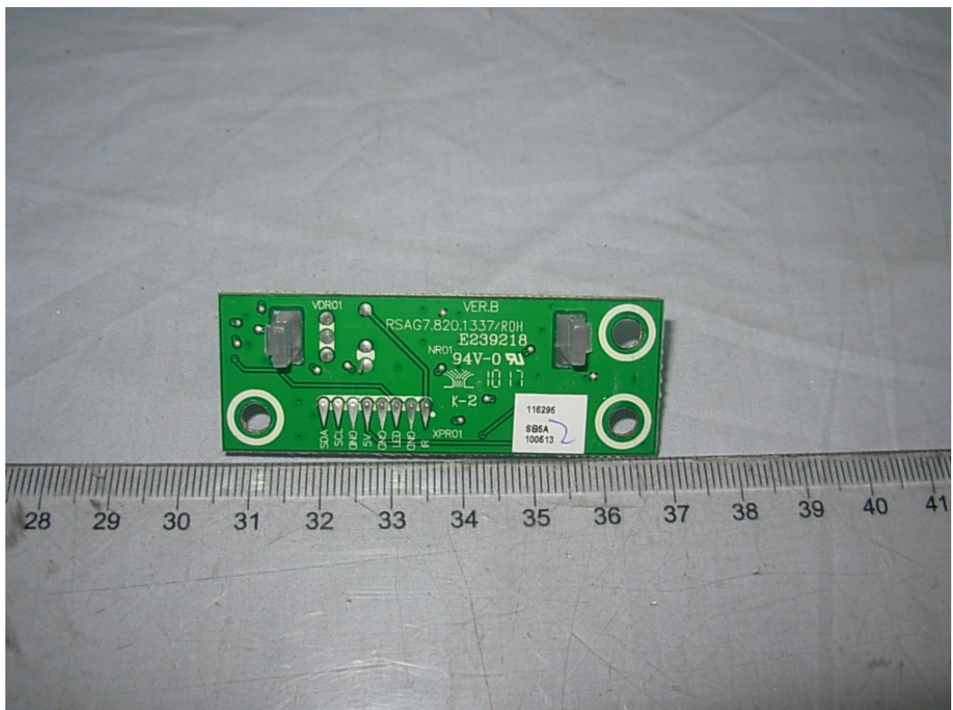
FIGURE 13 LCD TV (M/N: LTDN37W60MH) IR BOARD (SOLDERED SIDE)
