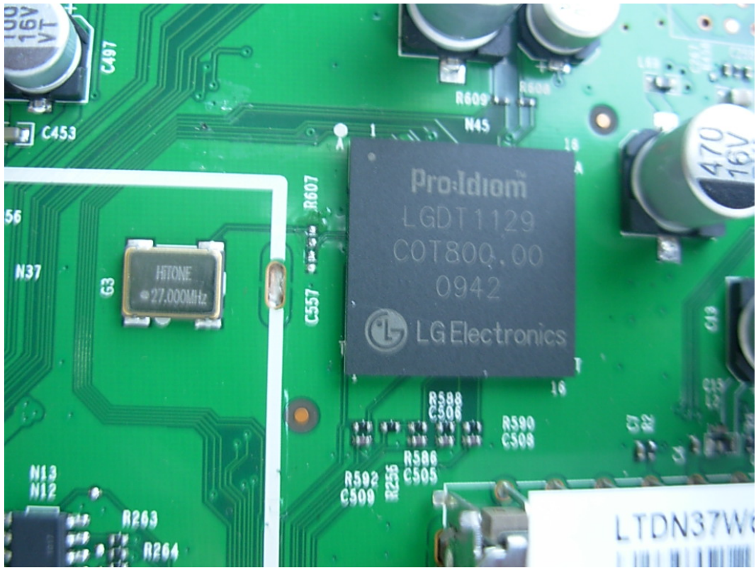
FIGURE 7 LCD TV (M/N: LTDN37W60MH) CRYSTAL 1 & CHIP 1 ON MAIN BOARD
