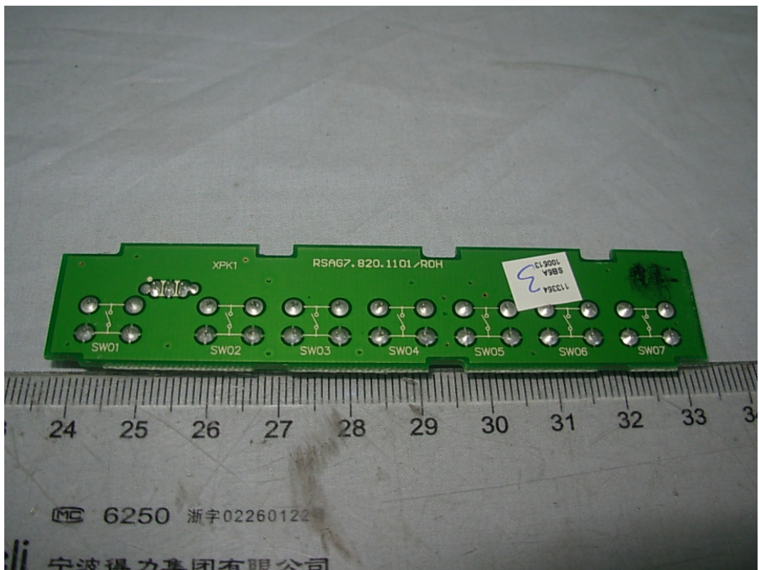
FIGURE 15 LCD TV (M/N: LTDN37W60MH) KEY BOARD (SOLDERED SIDE)
