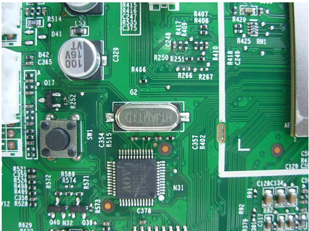
FIGURE 8 LCD TV (M/N: LTDN37W60MH) CRYSTAL 2 ON MAIN BOARD
