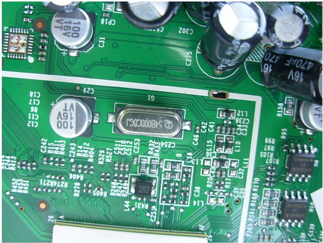
FIGURE 9 LCD TV (M/N: LTDN37W60MH) CRYSTAL 3 ON MAIN BOARD
