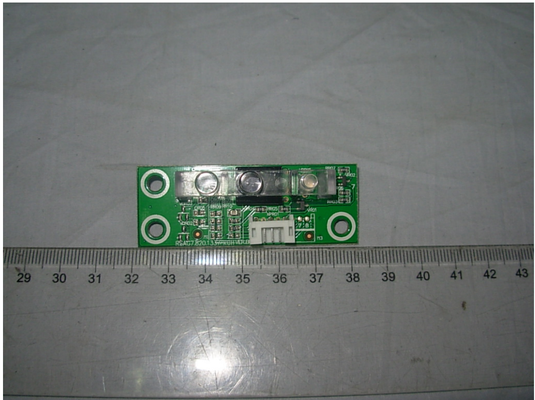
FIGURE 12 LCD TV (M/N: LTDN37W60MH) IR BOARD (COMPONENT SIDE)
