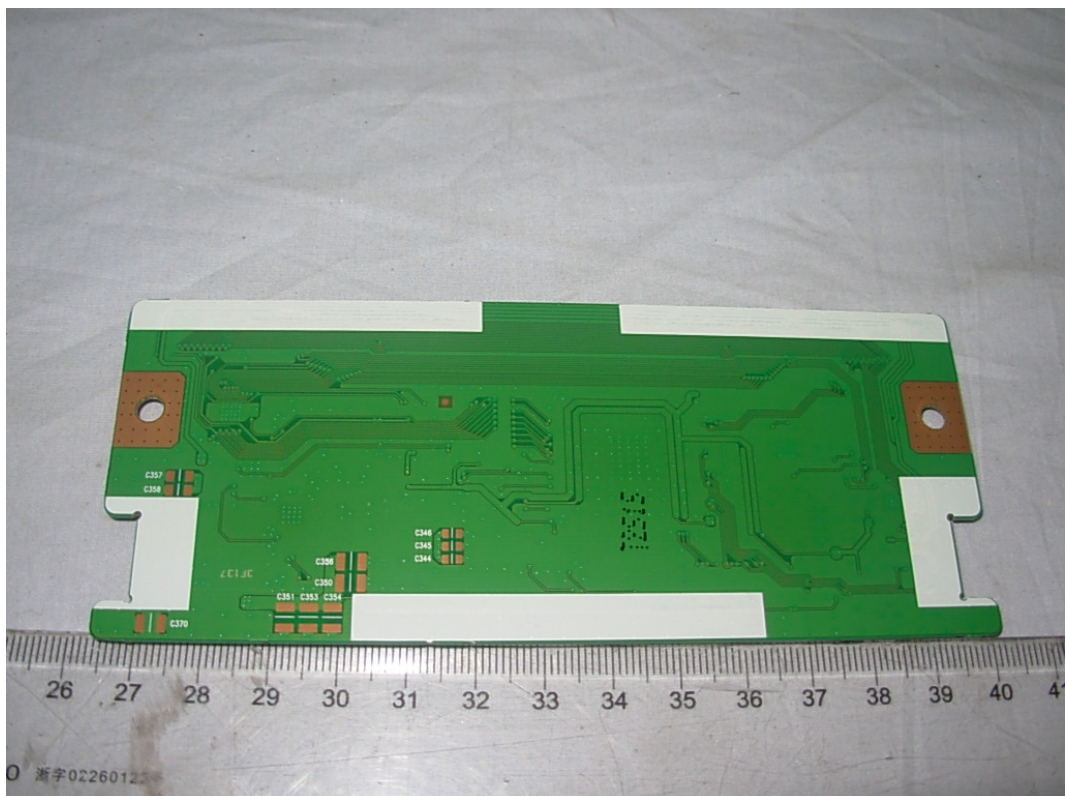
FIGURE 19 LCD TV (M/N: LTDN37W60MH) DISPLAY BOARD (SOLDERED SIDE)
