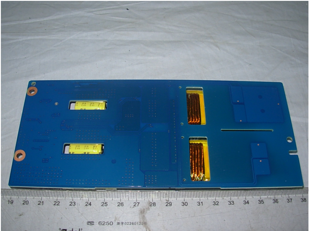
FIGURE 17 LCD TV (M/N: LTDN37W60MH) HIGH VOLTAGE SIGNAL BOARD (SOLDERED SIDE)
