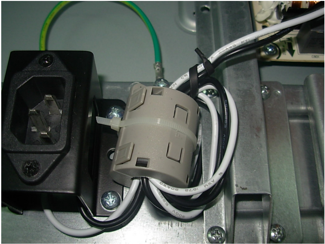
FIGURE 22 LCD TV (M/N: LTDN37W60MH) DEBUG#3
