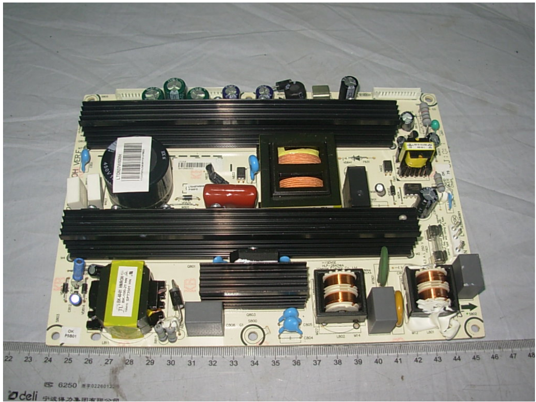
FIGURE 3 LCD TV (M/N: LTDN37W60MH) POWER BOARD (COMPONENT SIDE)
