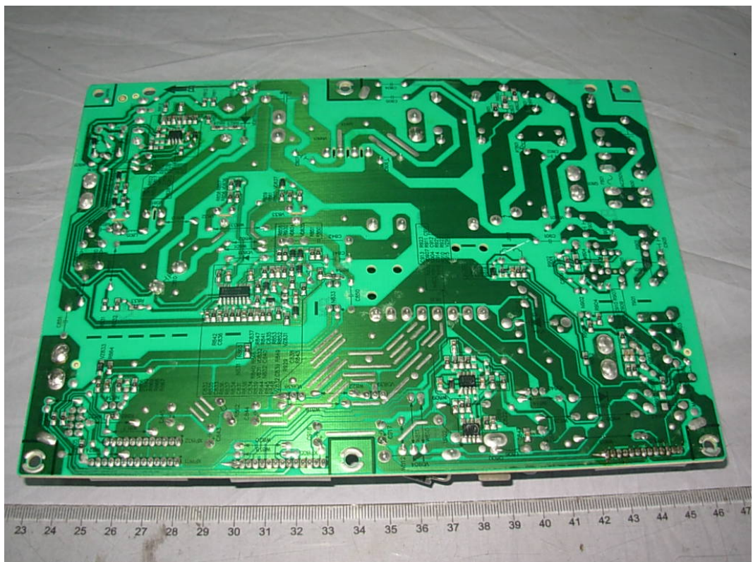
FIGURE 4 LCD TV (M/N: LTDN37W60MH) POWER BOARD (SOLDERED SIDE)
