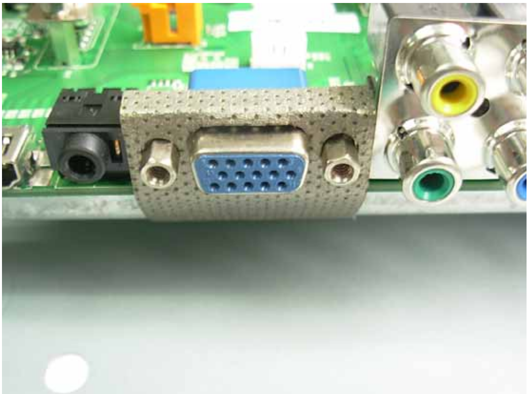
FIGURE 18 LCD TV (M/N: LHDN32V87HUS) DEBUG #3
