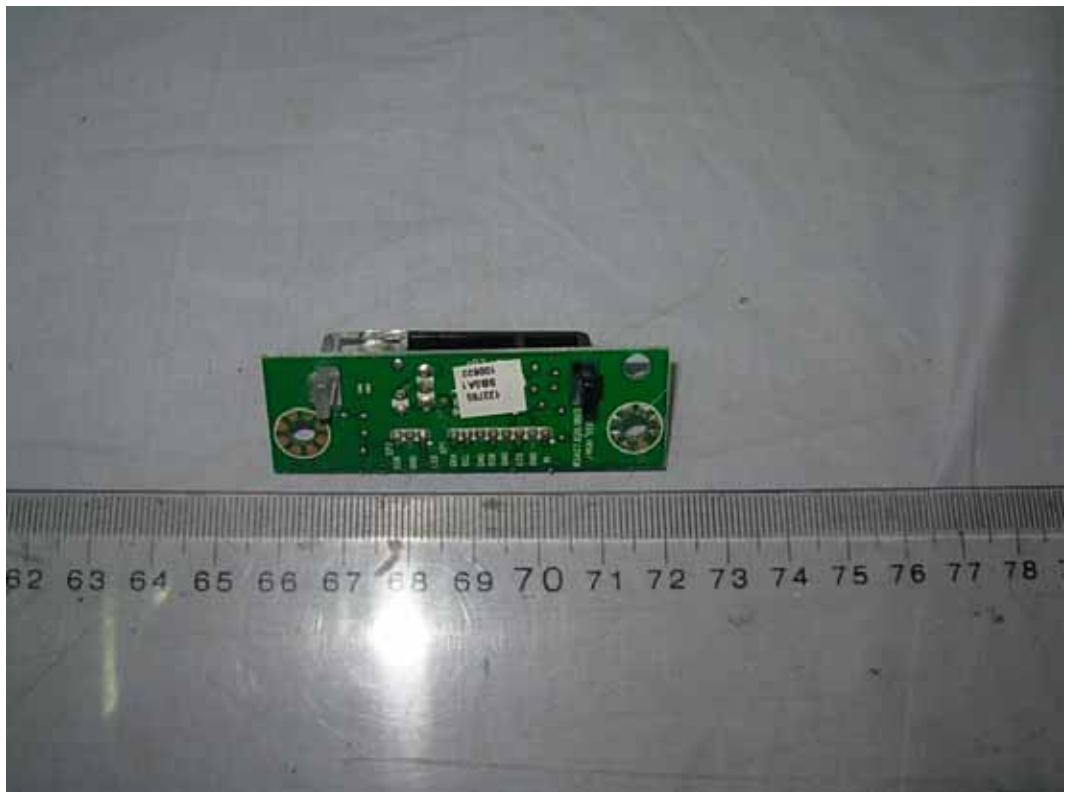
FIGURE 10 LCD TV (M/N: LHDN32V87HUS) IR BOARD (SOLDERED SIDE)
