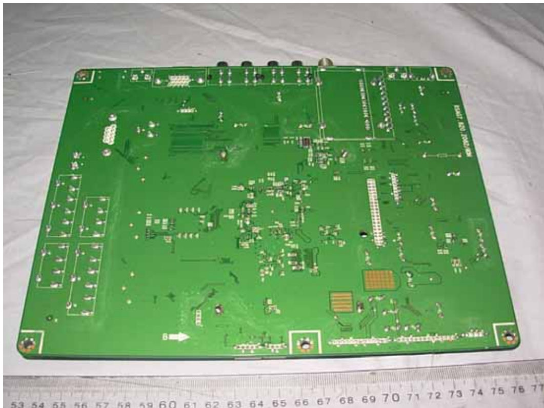
FIGURE 5 LCD TV (M/N: LHDN32V87HUS) MAIN BOARD (SOLDERED SIDE)
