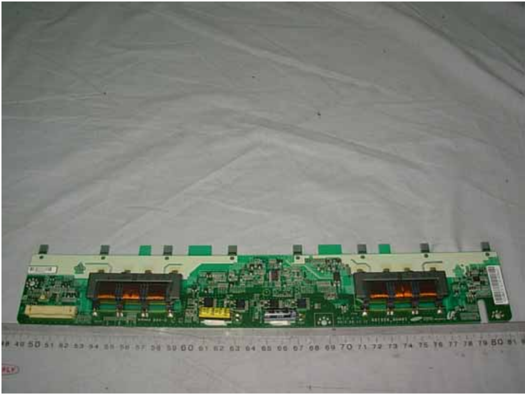
FIGURE 13 LCD TV (M/N: LHDN32V87HUS) HIGH VOLTAGE SIGNAL BOARD (COMPONENT SIDE)
