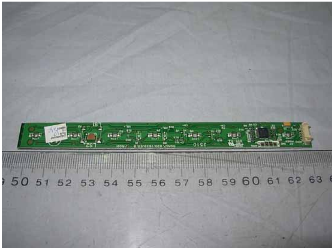
FIGURE 11 LCD TV (M/N: LHDN32V87HUS) KEY BOARD (COMPONENT SIDE)
