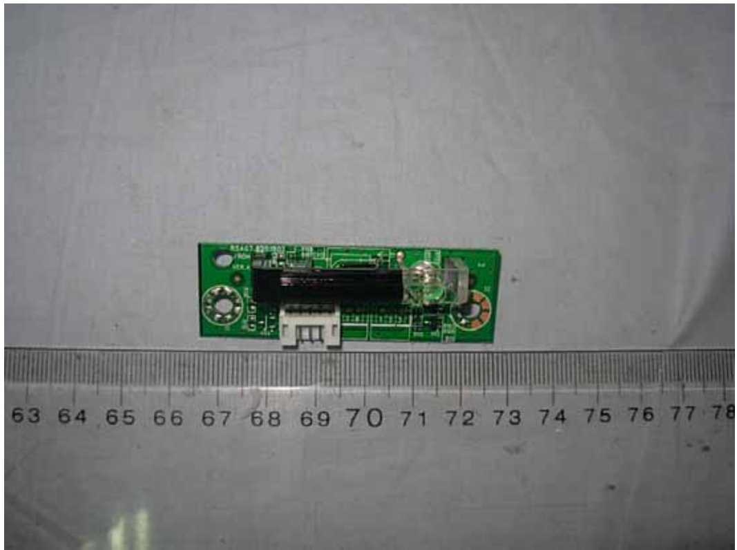
FIGURE 9 LCD TV (M/N: LHDN32V87HUS) IR BOARD (COMPONENT SIDE)
