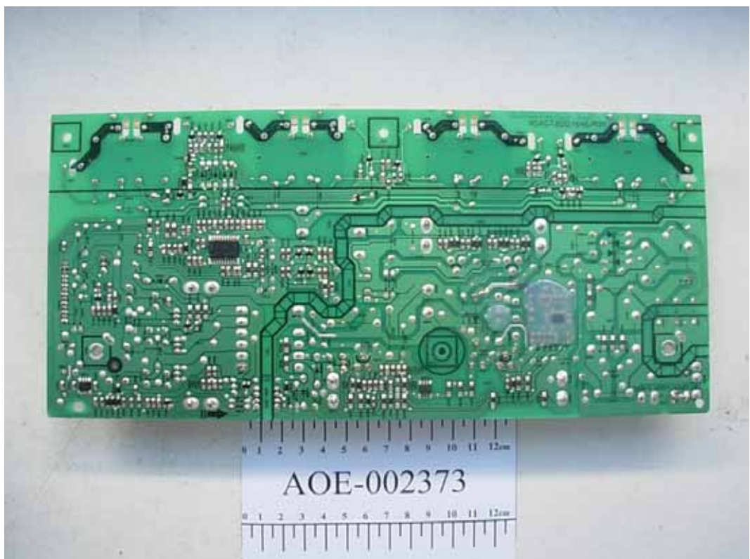
FIGURE 8 LCD TV (M/N: ELCHS262) POWER BOARD (SOLDERED SIDE)
