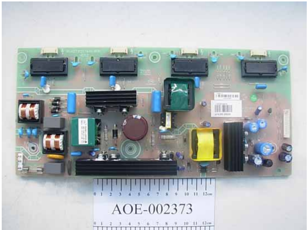
FIGURE 7 LCD TV (M/N: ELCHS262) POWER BOARD (COMPONENT SIDE)
