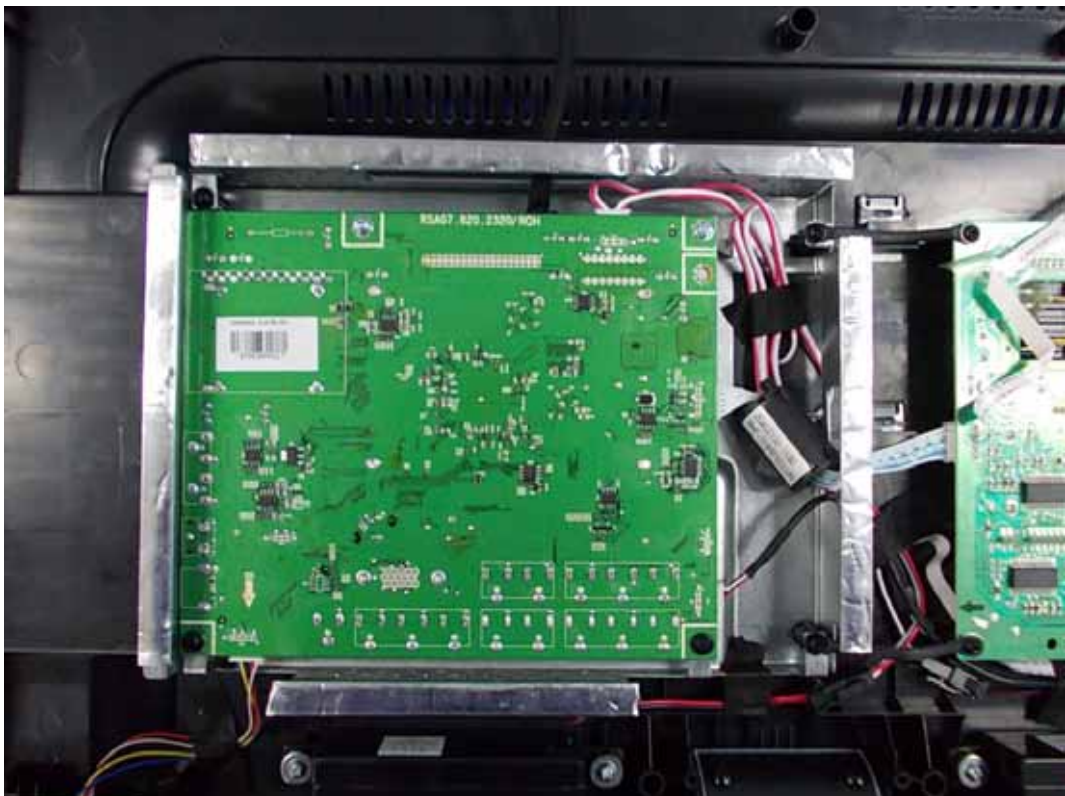
FIGURE 15 LCD TV (M/N: LTDN24K20US) DEBUG 2
