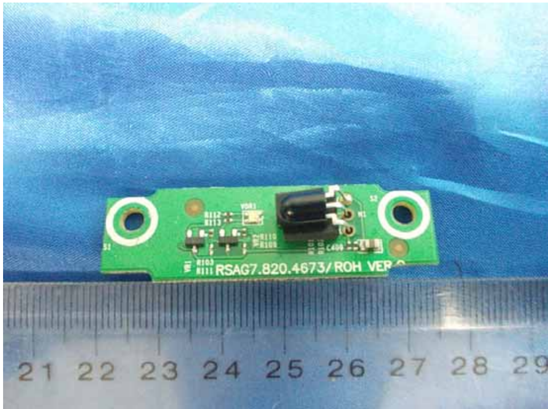
FIGURE 10 LCD TV (M/N: LTDN24K20US) IR BOARD (COMPONENT SIDE)
