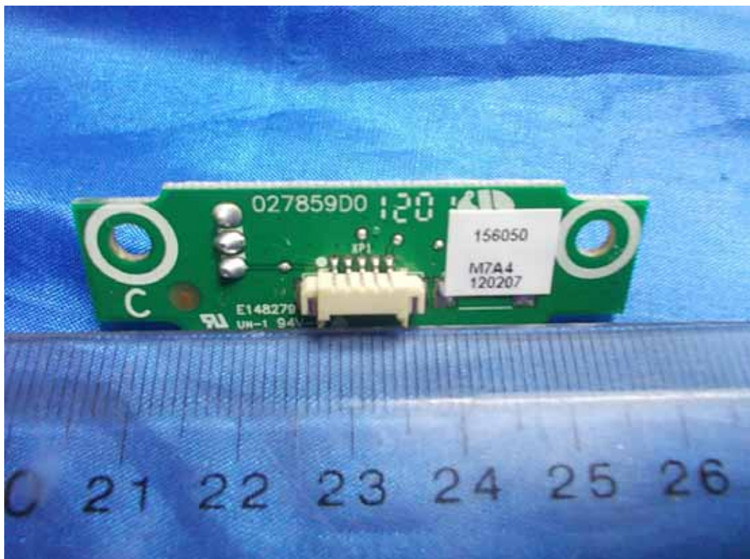
FIGURE 11 LCD TV (M/N: LTDN24K20US) IR BOARD (SOLDERED SIDE)
