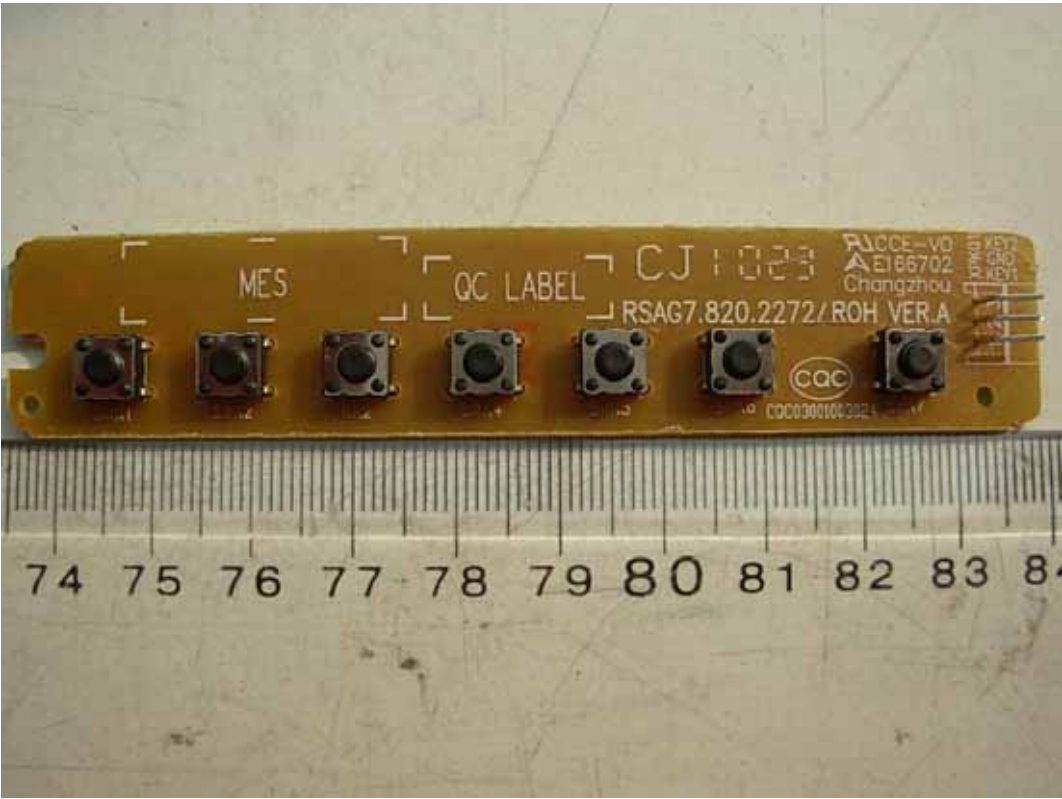
FIGURE 11 LCD TV (M/N: LEDN24K15PUS) KEY BOARD (COMPONENT SIDE)
