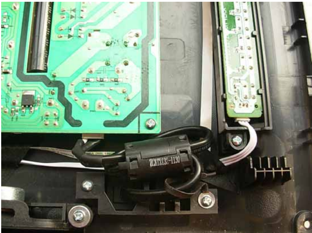
FIGURE 16 LCD TV (M/N: LEDN24K15PUS) DEBUG 2
