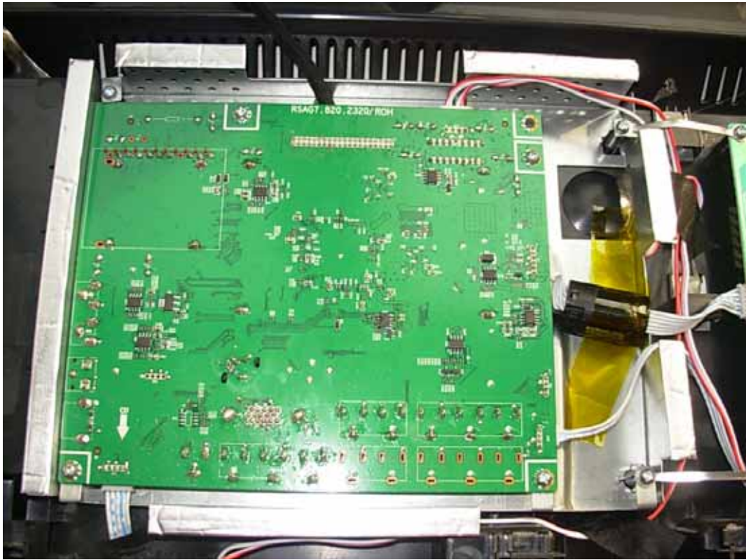
FIGURE 17 LCD TV (M/N: LEDN24K15PUS) DEBUG 3
