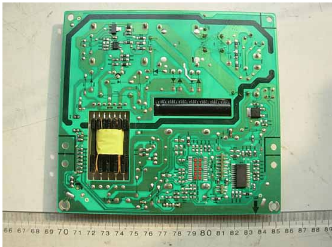
FIGURE 4 LCD TV (M/N: LEDN24K15PUS) POWER BOARD (SOLDERED SIDE)
