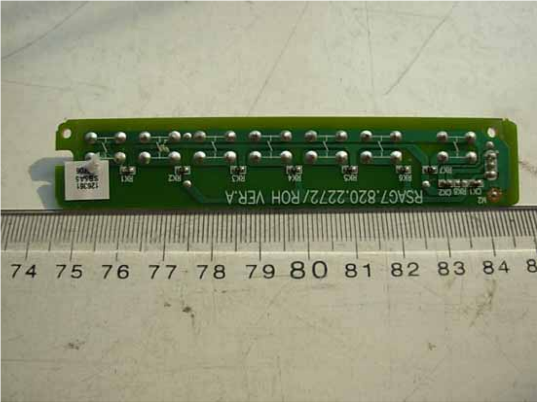
FIGURE 12 LCD TV (M/N: LEDN24K15PUS) KEY BOARD (SOLDERED SIDE)
