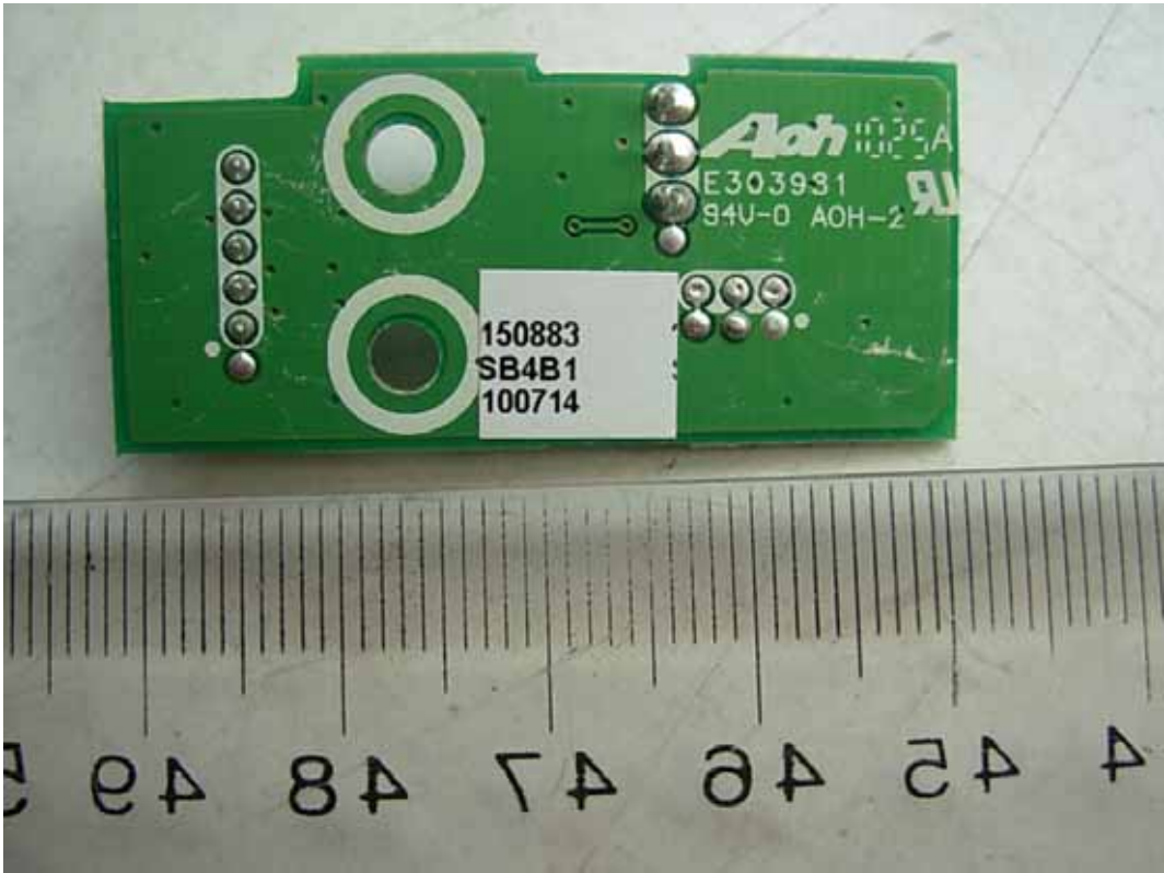
FIGURE 10 LCD TV (M/N: LEDN24K15PUS) IR BOARD (SOLDERED SIDE)
