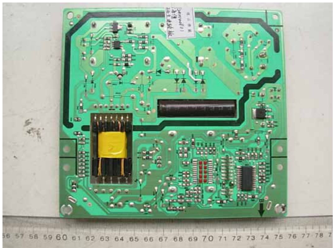
FIGURE 4 LCD TV (M/N: LEDN24K15PAM) POWER BOARD (SOLDERED SIDE)
