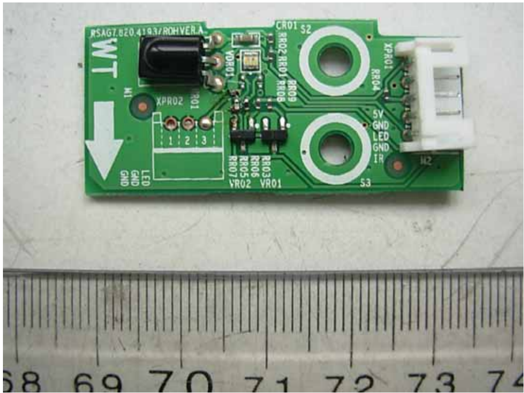
FIGURE 9 LCD TV (M/N: LEDN24K15PAM) IR BOARD (COMPONENT SIDE)
