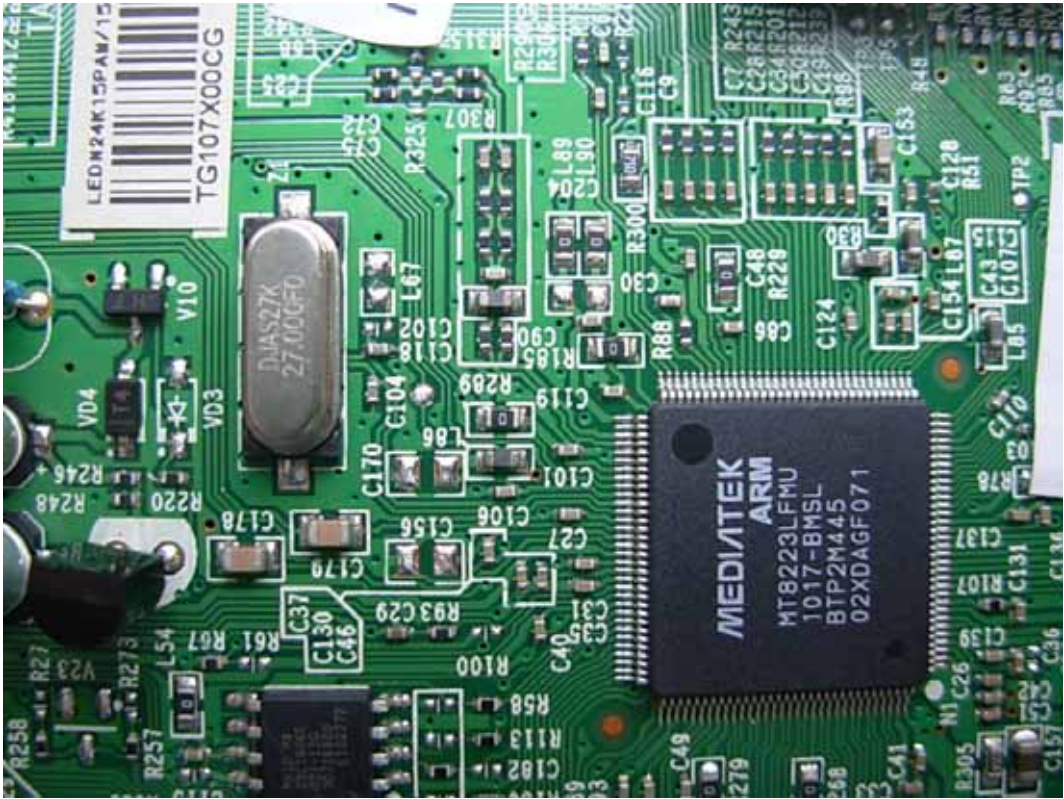
FIGURE 7 LCD TV (M/N: LEDN24K15PAM) CRYSTAL & CHIP ON MAIN BOARD
