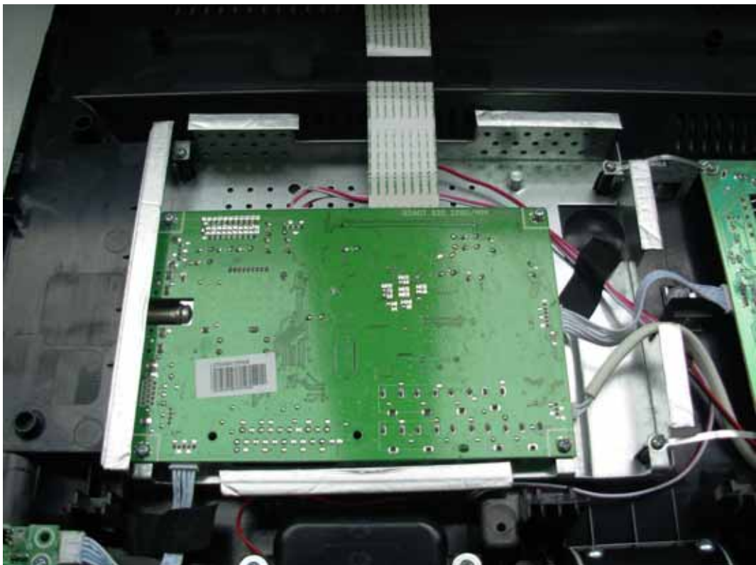
FIGURE 16 LCD TV (M/N: LEDN24K15PAM) DEBUG 2
