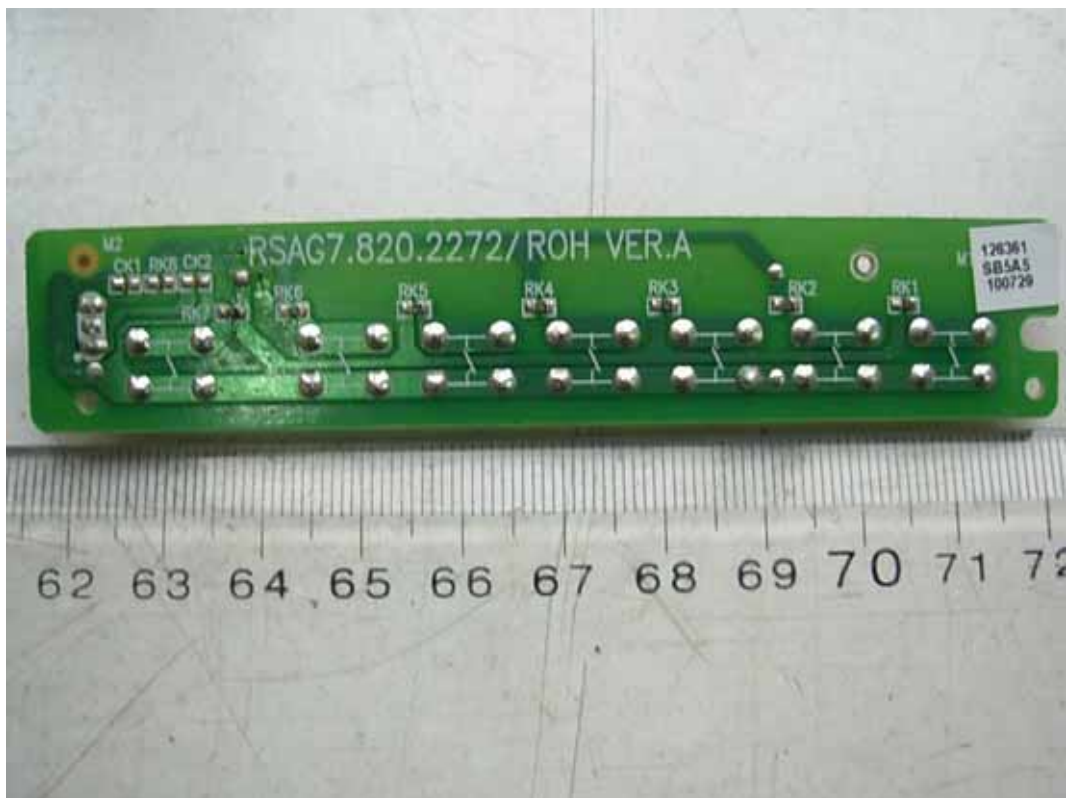
FIGURE 12 LCD TV (M/N: LEDN24K15PAM) KEY BOARD (SOLDERED SIDE)
