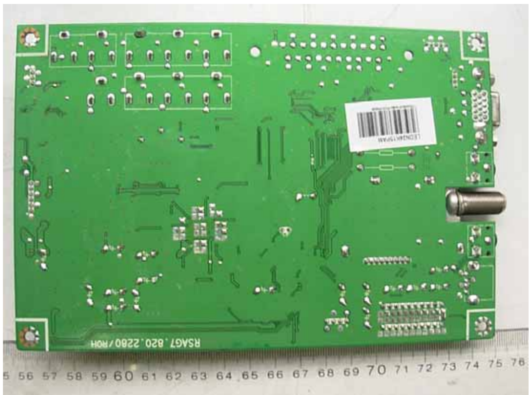
FIGURE 6 LCD TV (M/N: LEDN24K15PAM) MAIN BOARD (SOLDERED SIDE)
