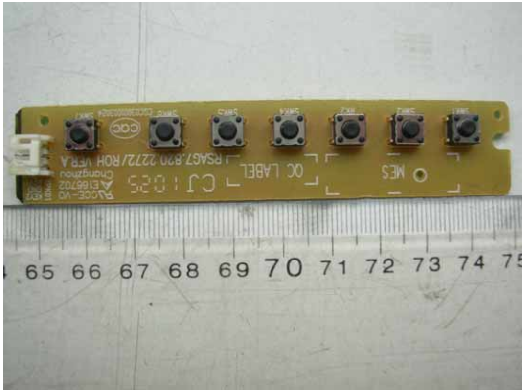
FIGURE 11 LCD TV (M/N: LEDN24K15PAM) KEY BOARD (COMPONENT SIDE)
