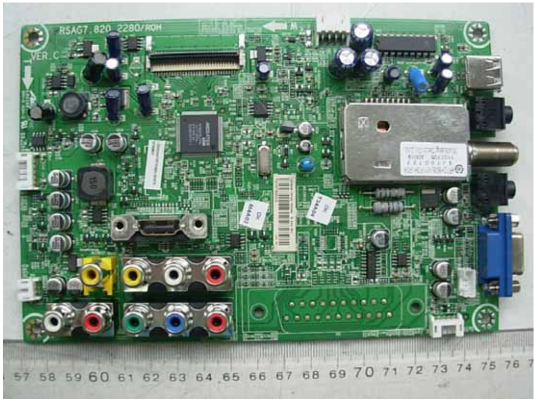
FIGURE 5 LCD TV (M/N: LEDN24K15PAM) MAIN BOARD (COMPONENT SIDE)
