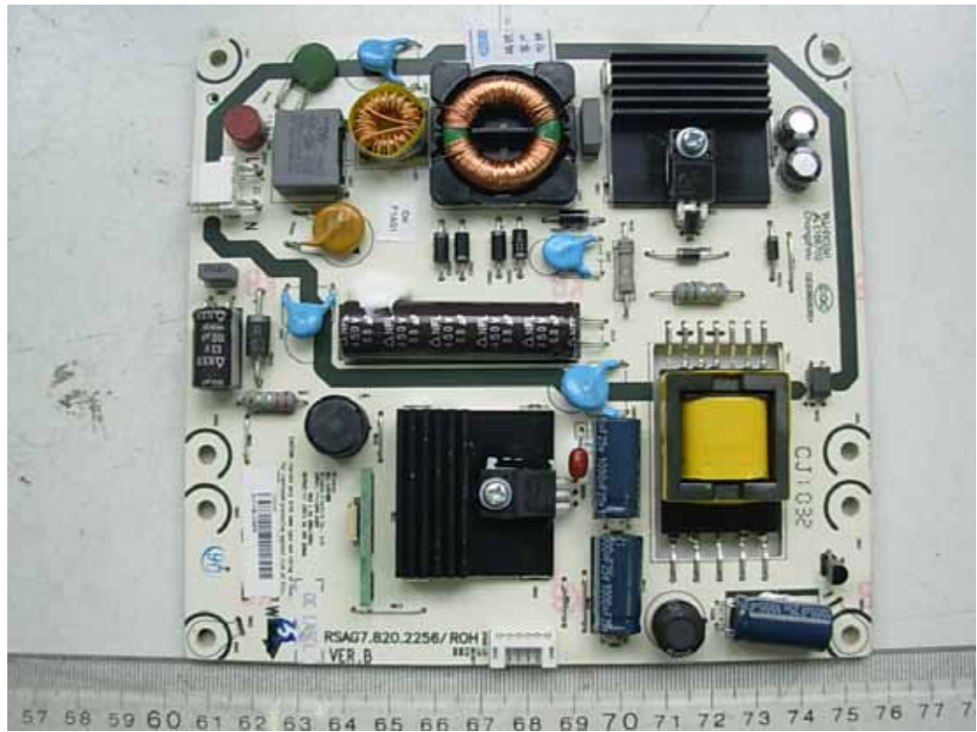
FIGURE 3 LCD TV (M/N: LEDN24K15PAM) POWER BOARD (COMPONENT SIDE)
