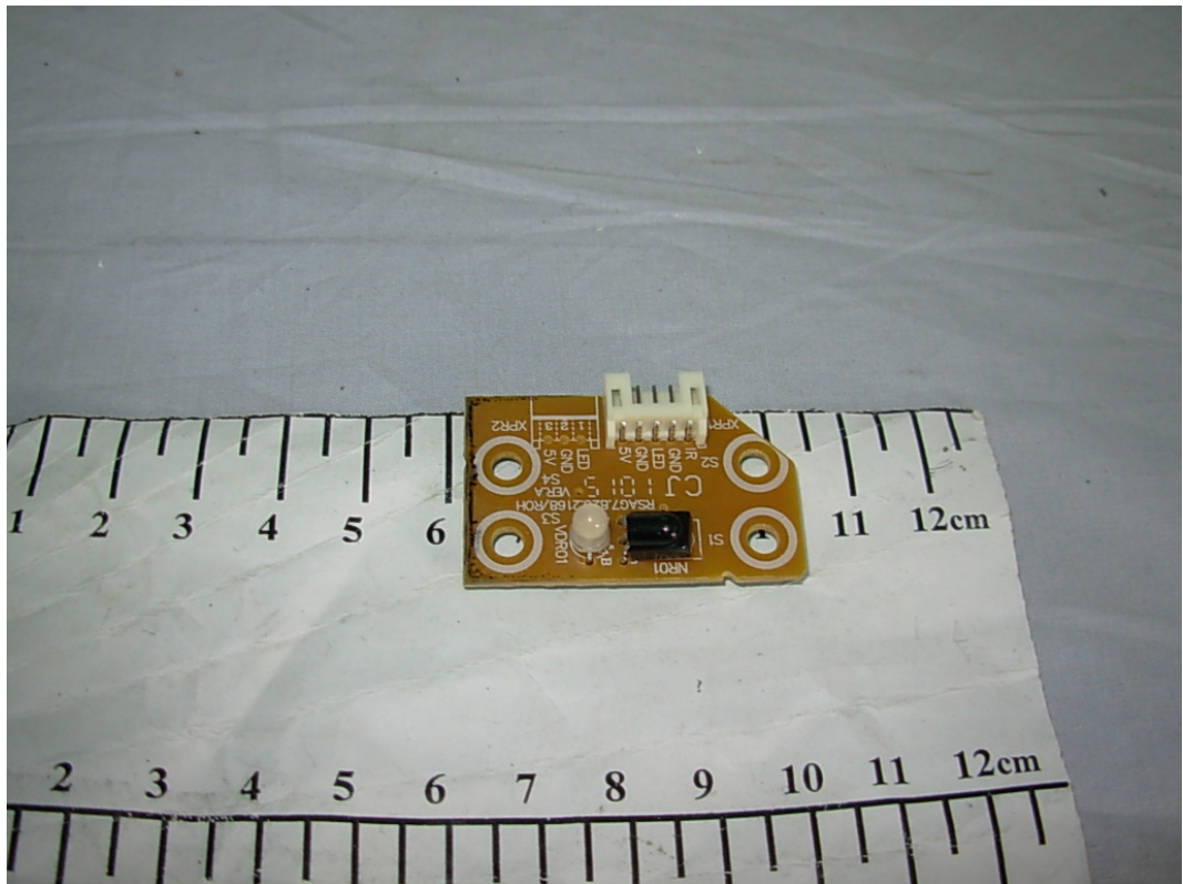
FIGURE 8 LCD TV (M/N: LTDN24V86NUS) IR BOARD (COMPONENT SIDE)
