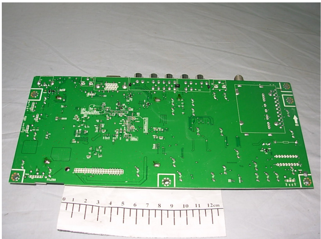
FIGURE 5 LCD TV (M/N: LTDN24V86NUS) MAIN BOARD (SOLDERED SIDE)
