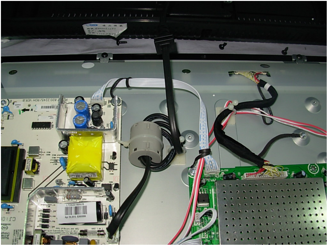
FIGURE 15 LCD TV (M/N: LTDN24V86NUS) DEBUG
