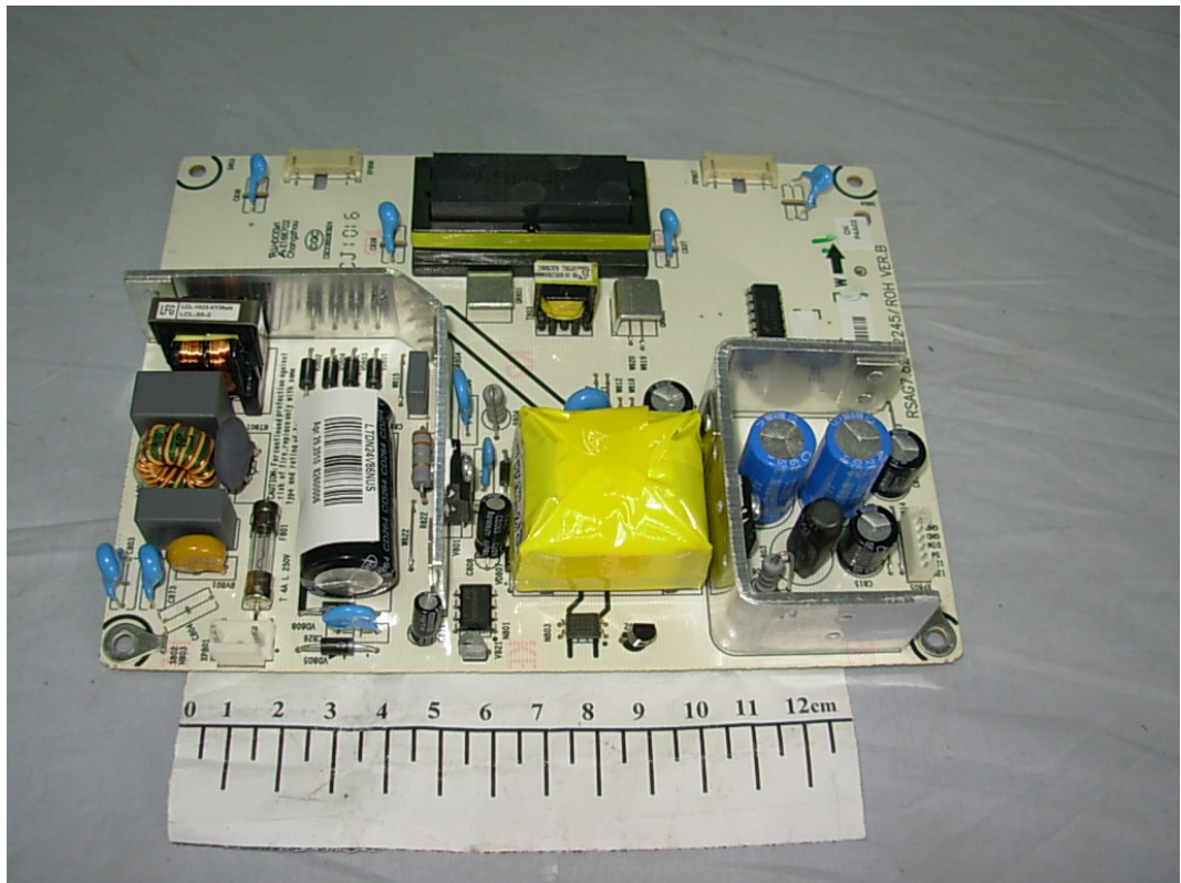
FIGURE 2 LCD TV (M/N: LTDN24V86NUS) POWER BOARD (COMPONENT SIDE)
