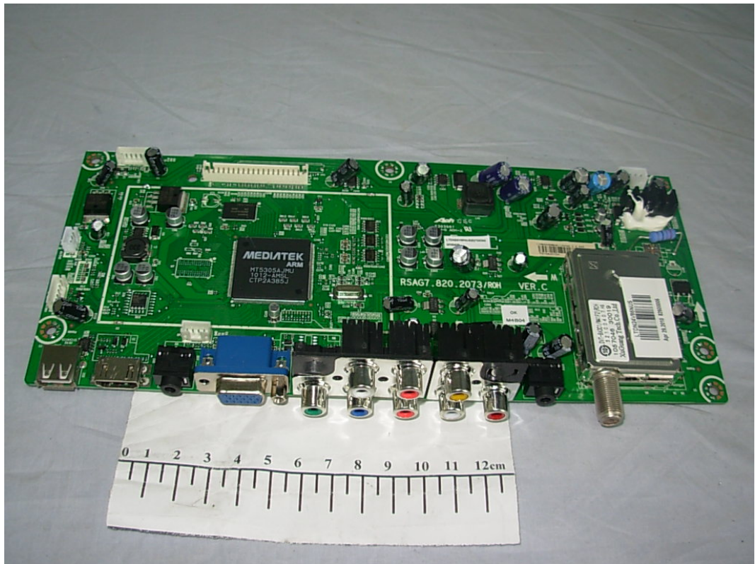
FIGURE 4 LCD TV (M/N: LTDN24V86NUS) MAIN BOARD (COMPONENT SIDE)
