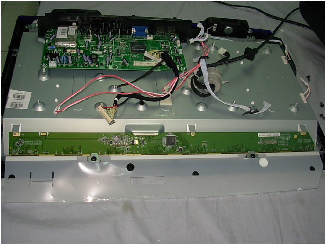
FIGURE 11 LCD TV (M/N: LTDN24V86NUS) LCD PANEL MAIN BOARD (COMPONENT SIDE)
