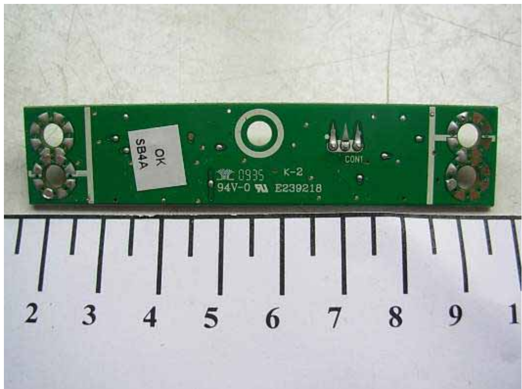
FIGURE 10 LCD TV (M/N: LTDN24V86US) LED BOARD (SOLDERED SIDE)
