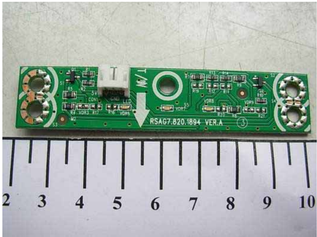
FIGURE 9 LCD TV (M/N: LTDN24V86US) LED BOARD (COMPONENT SIDE)
