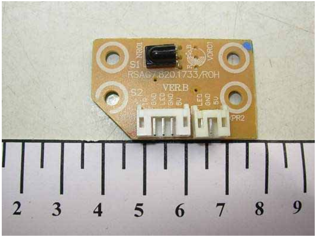
FIGURE 13 LCD TV (M/N: LTDN24V86US) IR BOARD (COMPONENT SIDE)
