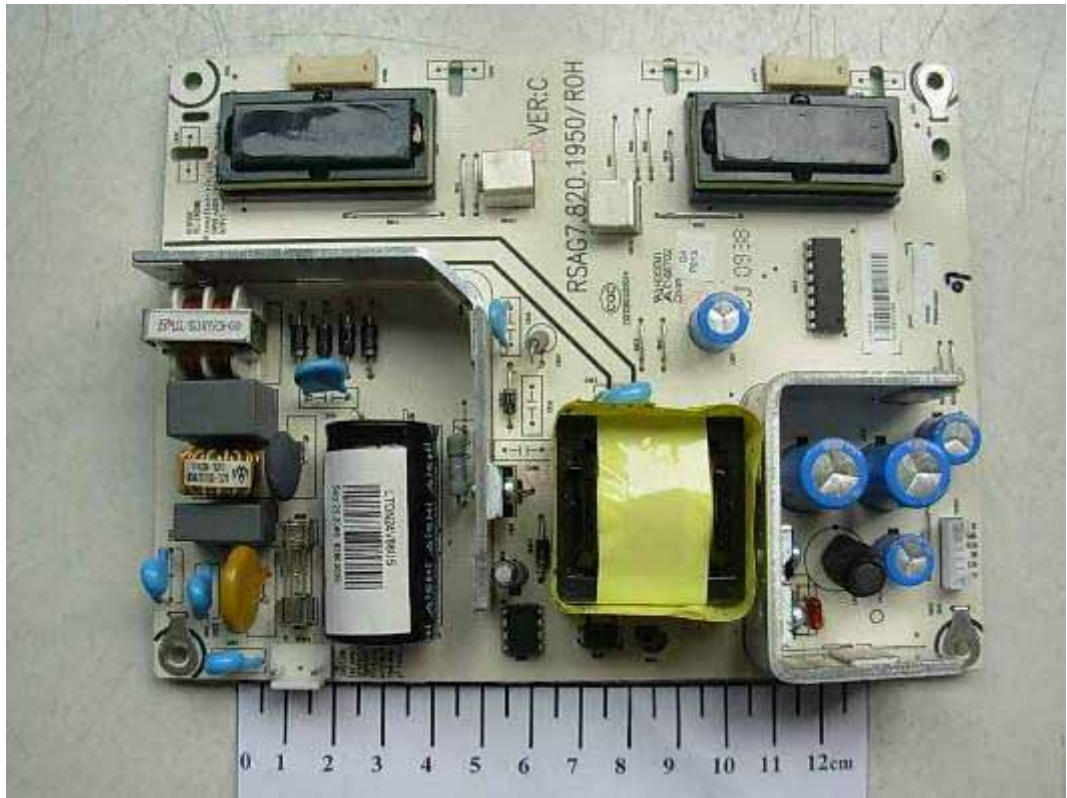
FIGURE 7 LCD TV (M/N: LTDN24V86US) POWER BOARD (COMPONENT SIDE)
