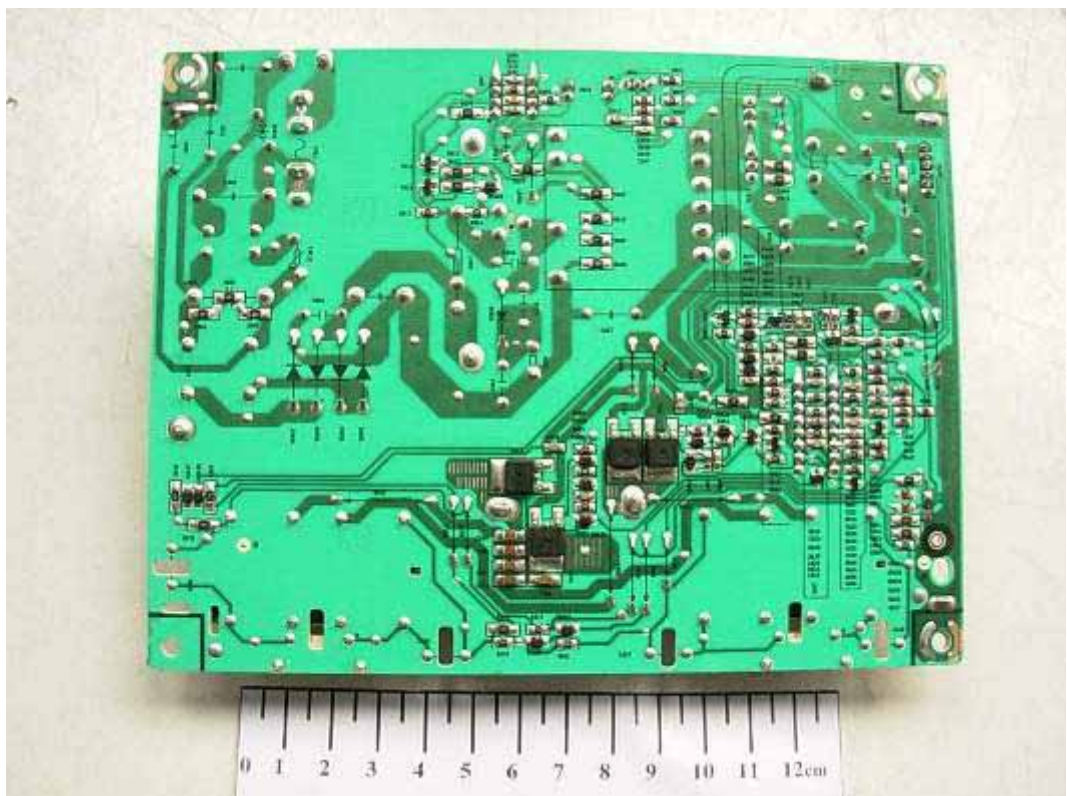
FIGURE 8 LCD TV (M/N: LTDN24V86US) POWER BOARD (SOLDERED SIDE)
