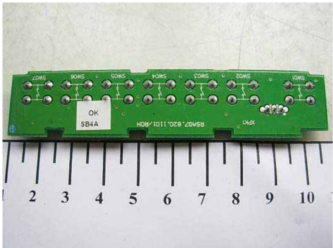
FIGURE 12 LCD TV (M/N: LTDN24V86US) KEY BOARD (SOLDERED SIDE)
