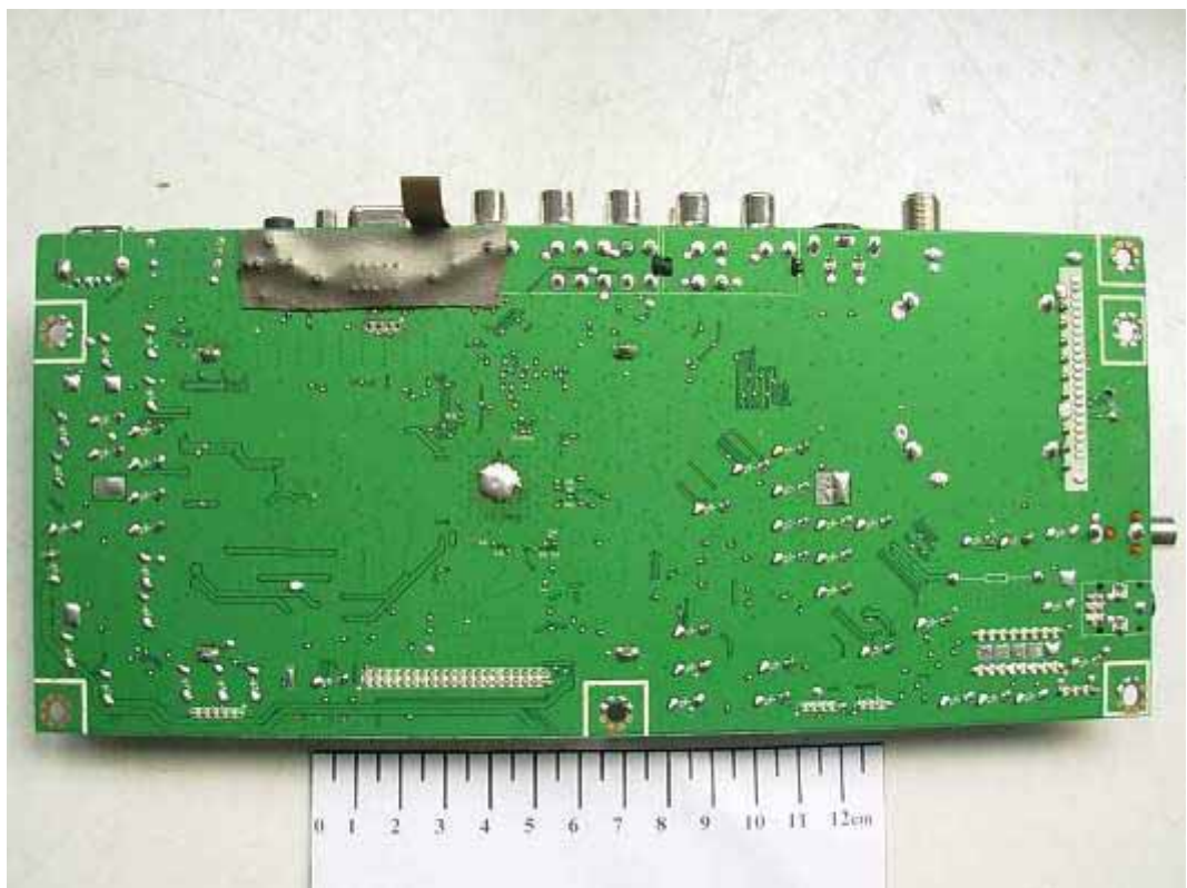
FIGURE 3 LCD TV (M/N: LTDN24V86US) MAIN BOARD (SOLDERED SIDE)
