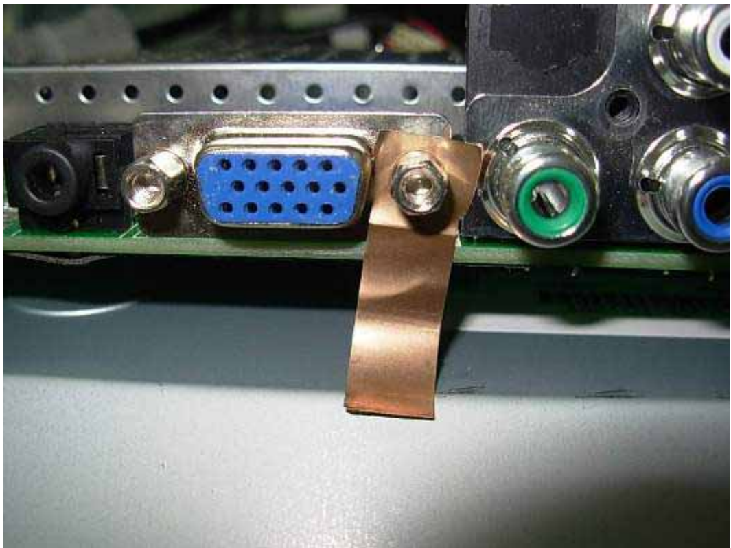
FIGURE 20 LCD TV (M/N: LTDN24V86US) DEBUG #3
