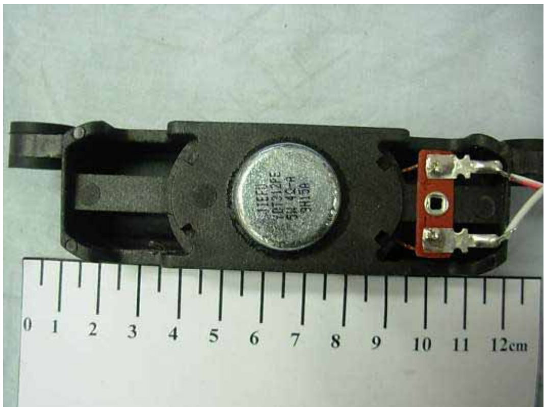
FIGURE 16 LCD TV (M/N: LTDN24V86US) SPEAKER BACK
