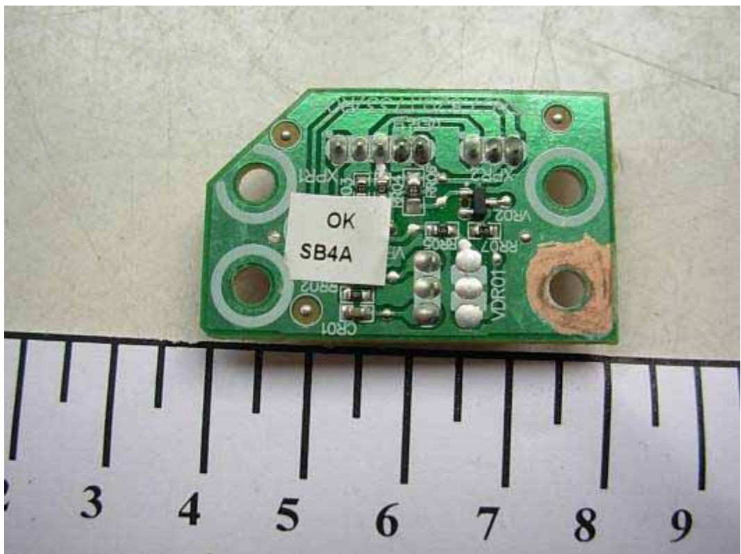
FIGURE 14 LCD TV (M/N: LTDN24V86US) IR BOARD (SOLDERED SIDE)
