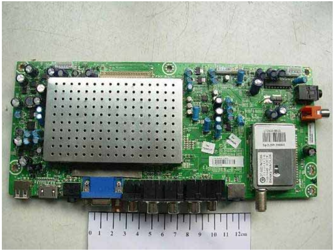
FIGURE 2 LCD TV (M/N: LTDN24V86US) MAIN BOARD (COMPONENT SIDE)
