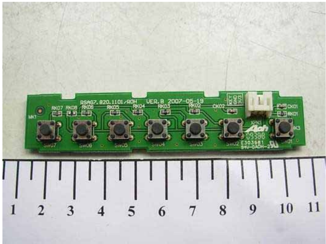
FIGURE 11 LCD TV (M/N: LTDN24V86US) KEY BOARD (COMPONENT SIDE)
