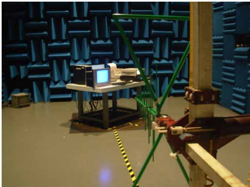
SETUP WITH MAXIMUM DETECTED EMISSION AT VERTICAL POLARIZATION (D-SUB 1360*768@60Hz)
