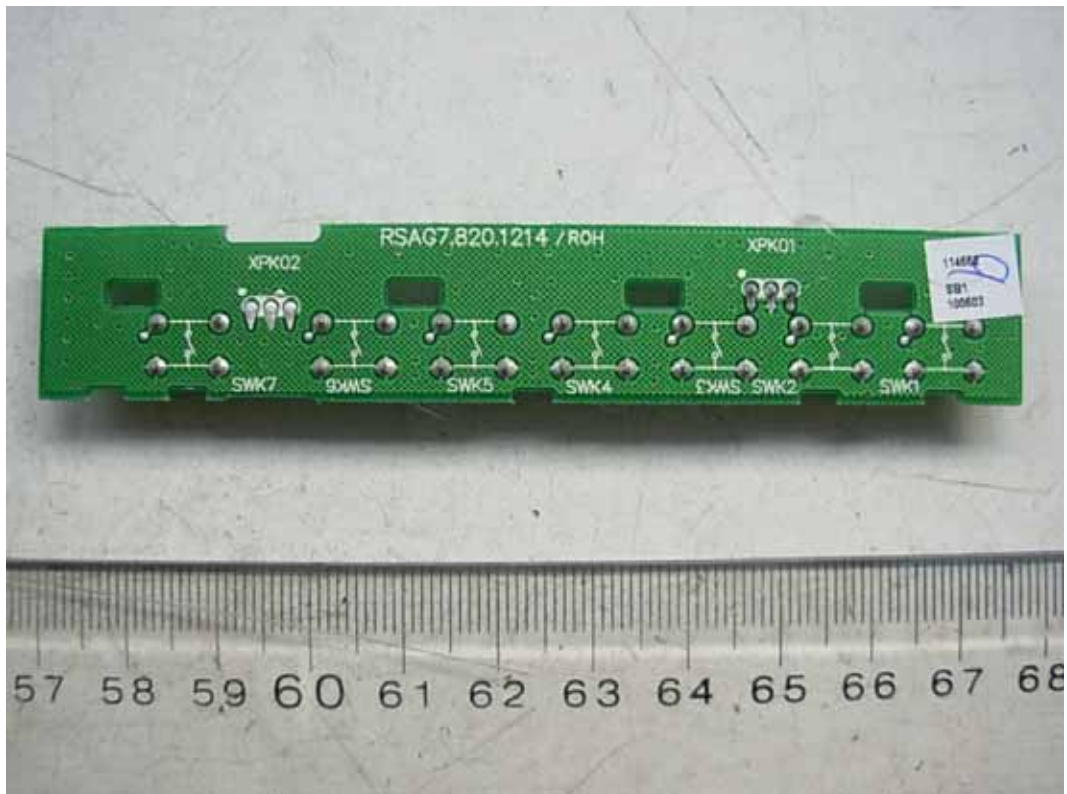
FIGURE 11 LCD TV (M/N: LCD19W57ACA) KEY BOARD (SOLDERED SIDE)
