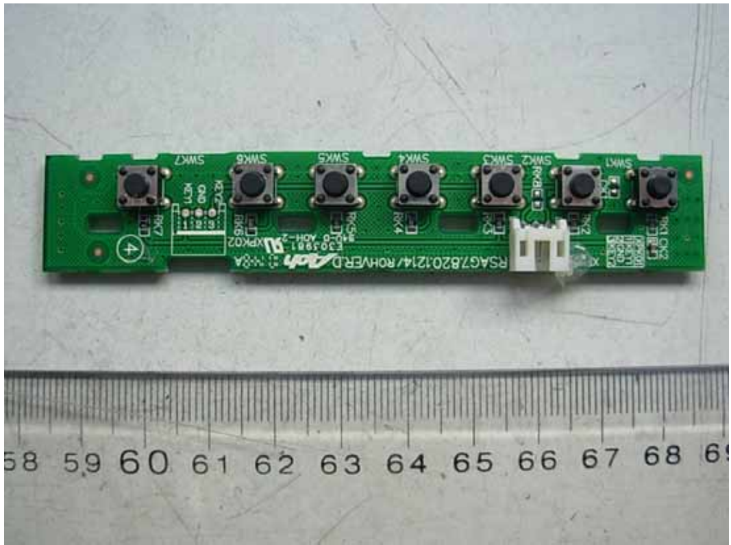
FIGURE 10 LCD TV (M/N: LCD19W57ACA) KEY BOARD (COMPONENT SIDE)
