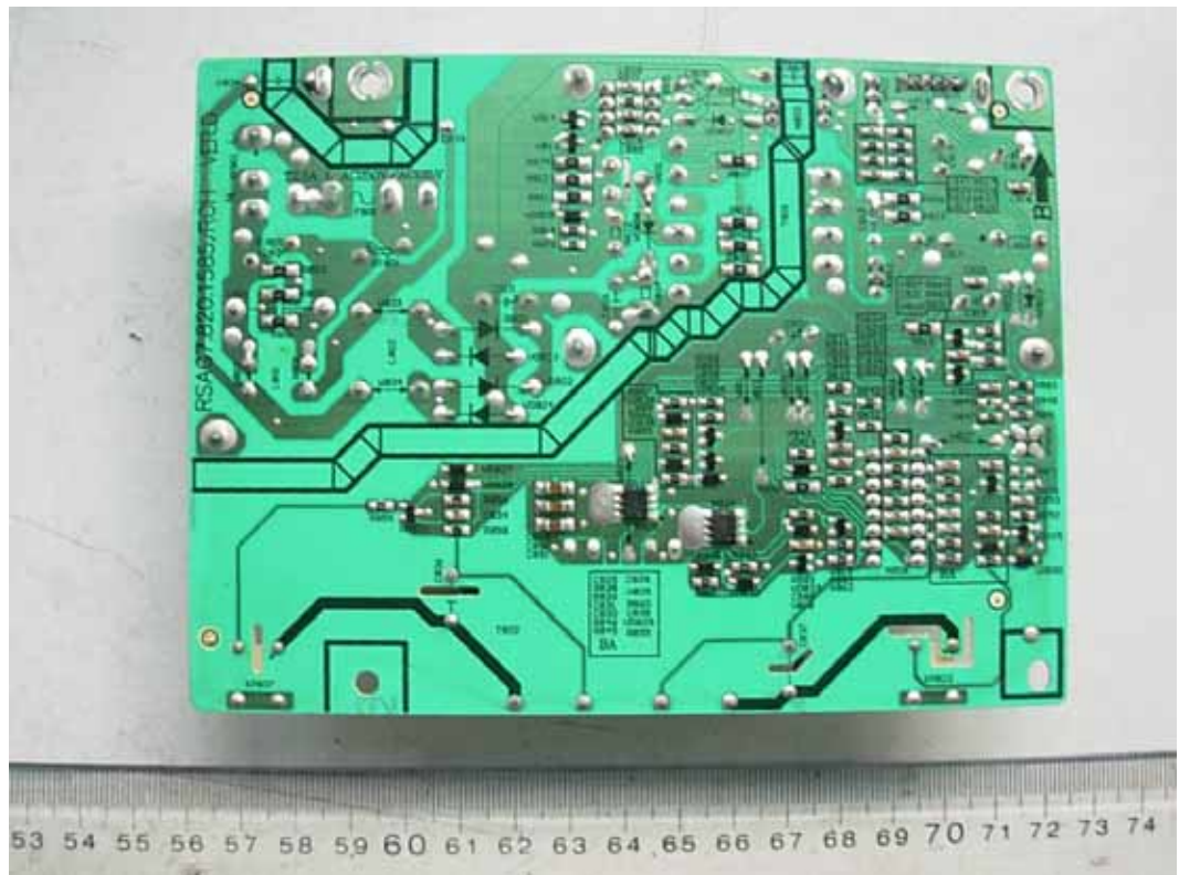
FIGURE 3 LCD TV (M/N: LCD19W57ACA) POWER BOARD (SOLDERED SIDE)
