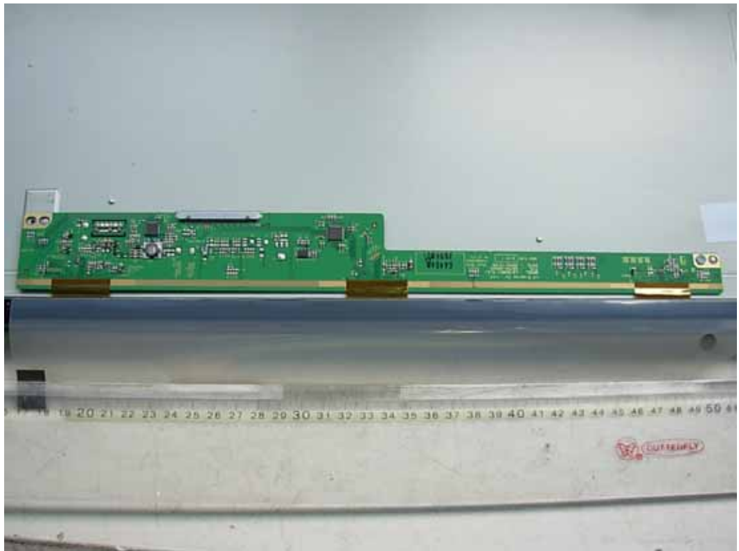
FIGURE 12 LCD TV (M/N: LCD19W57ACA) LCD PANEL MAIN BOARD (COMPONENT SIDE)
