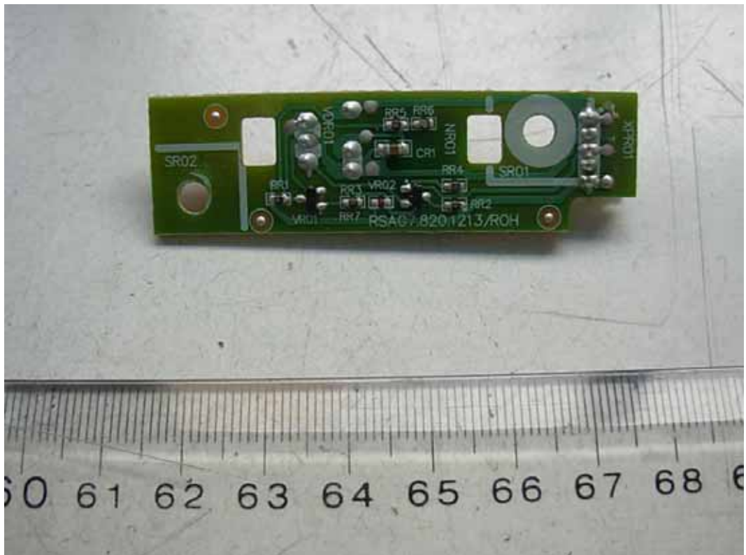
FIGURE 9 LCD TV (M/N: LCD19W57ACA) IR BOARD (SOLDERED SIDE)
