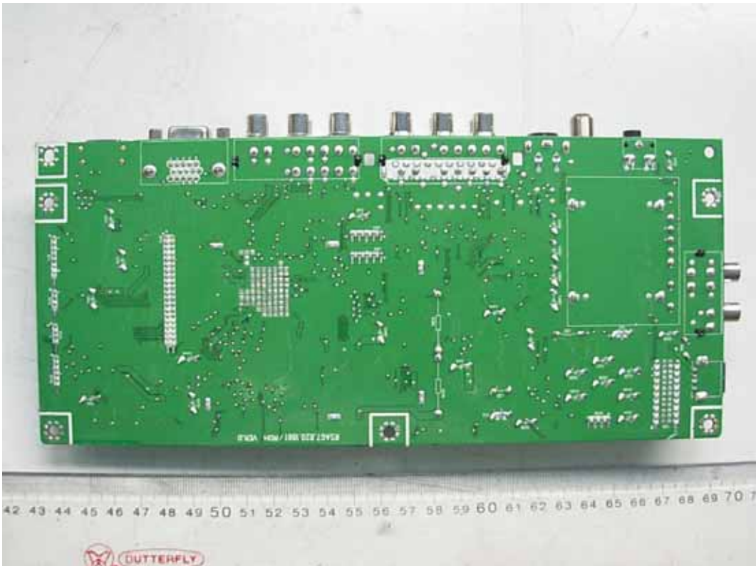
FIGURE 5 LCD TV (M/N: LCD19W57ACA) MAIN BOARD (SOLDERED SIDE)
