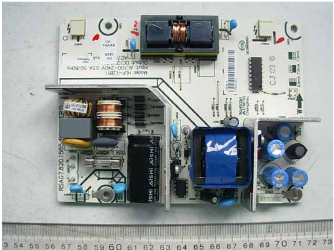
FIGURE 2 LCD TV (M/N: LCD19W57ACA) POWER BOARD (COMPONENT SIDE)
