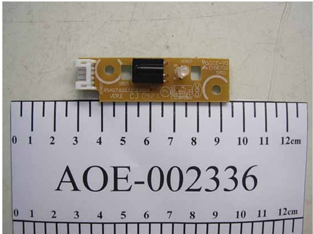
FIGURE 11 LCD TV (M/N: LCD19W57ACA) LED BOARD (COMPONENT SIDE)
