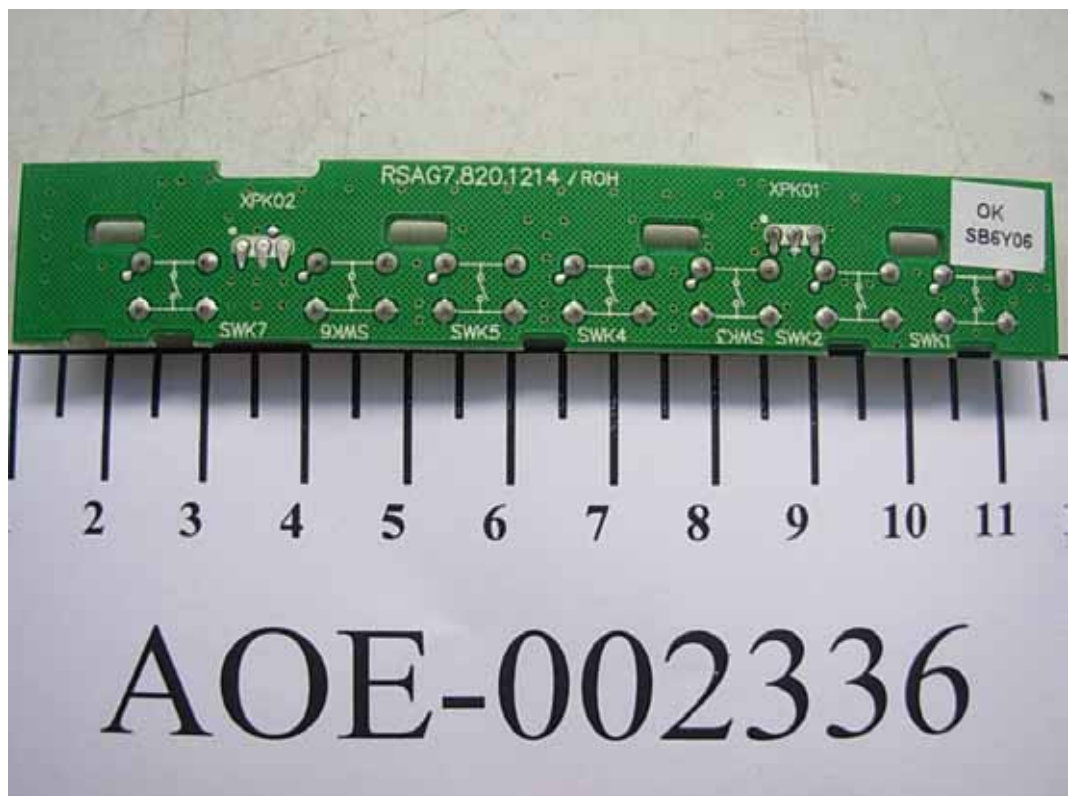
FIGURE 10 LCD TV (M/N: LCD19W57ACA) BUTTON BOARD (SOLDERED SIDE)
