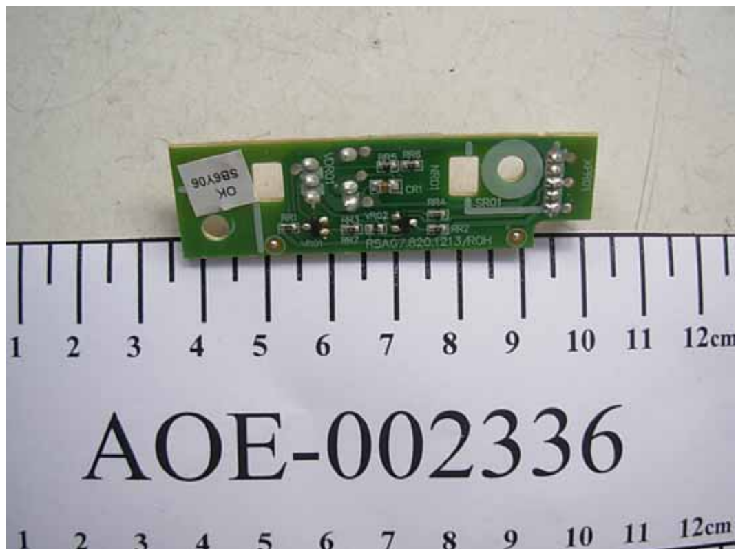
FIGURE 12 LCD TV (M/N: LCD19W57ACA) LED BOARD (SOLDERED SIDE)
