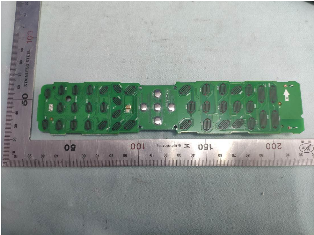
FIGURE 5 REMOTE CONTROL (M/N: ERF2A60(2002)) MAIN BOARD (SOLDERED SIDE)
