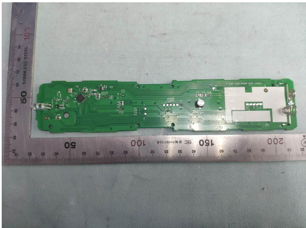
FIGURE 4 REMOTE CONTROL (M/N: ERF2A60(2002)) MAIN BOARD (COMPONENT SIDE)
