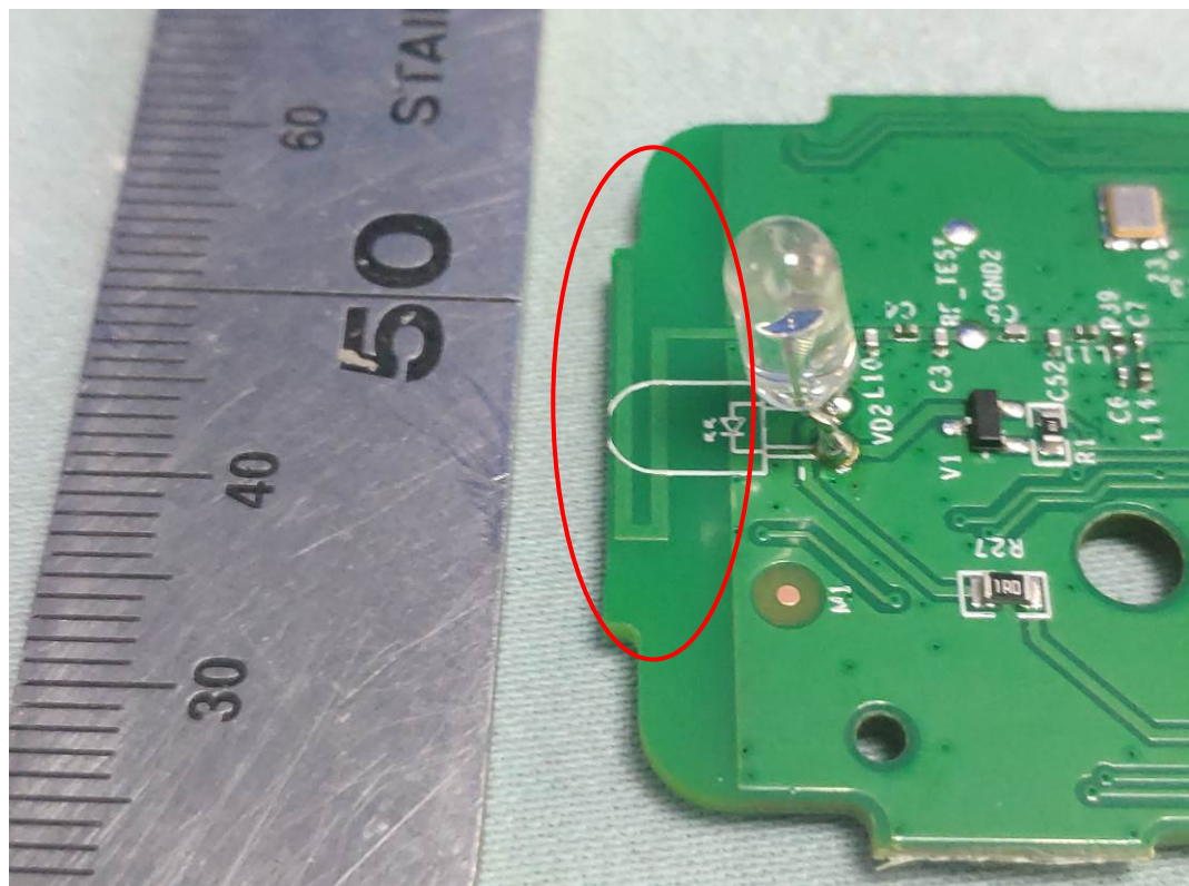
FIGURE 8 REMOTE CONTROL (M/N: ERF2A60(2002)) ANTENNA
