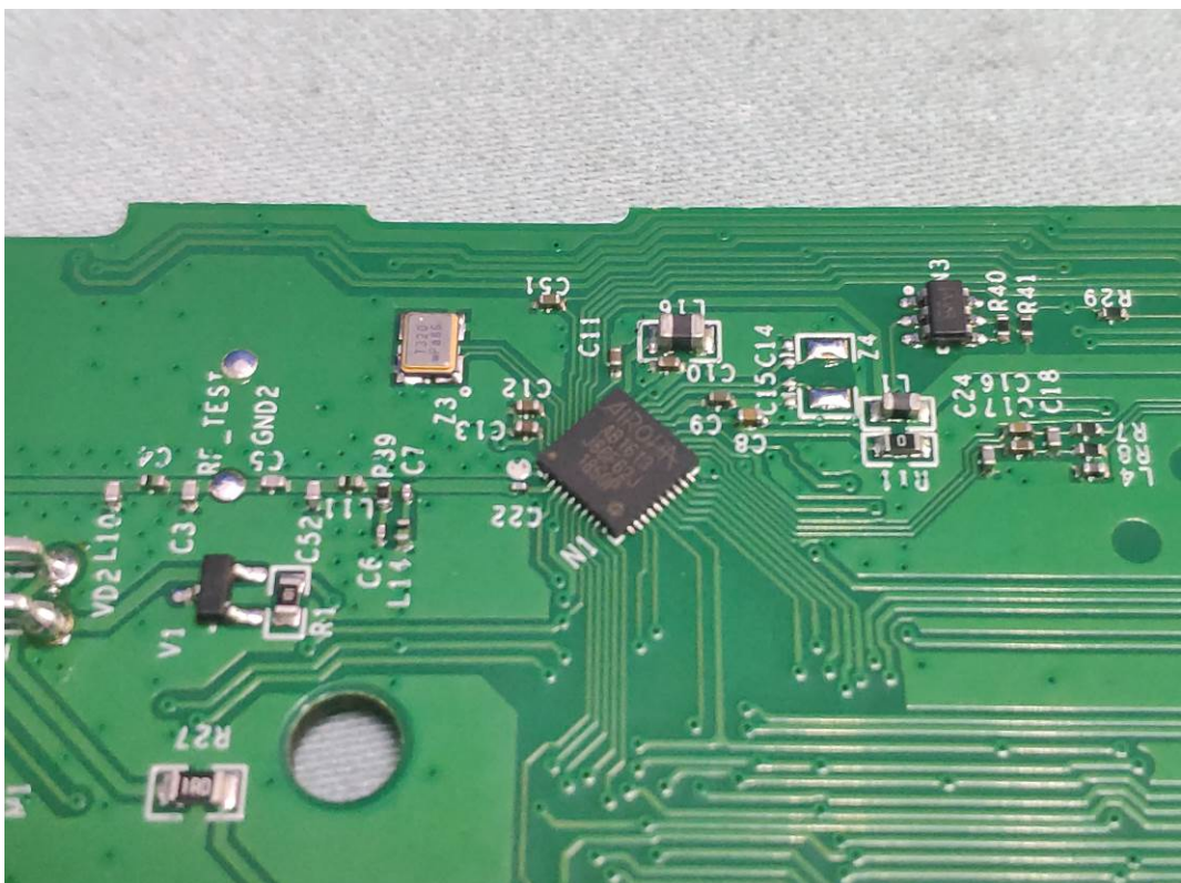
FIGURE 6 REMOTE CONTROL (M/N: ERF2A60(2002)) CHIP & CRYSTAL ON MAIN BOARD
