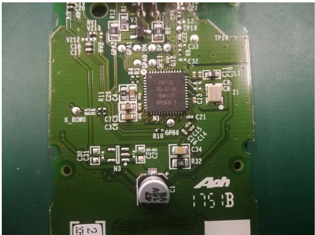
FIGURE 6 TV REMOTE CONTROL (M/N: ERF3A69) CHIP & CRYSTAL ON MAIN BOARD
