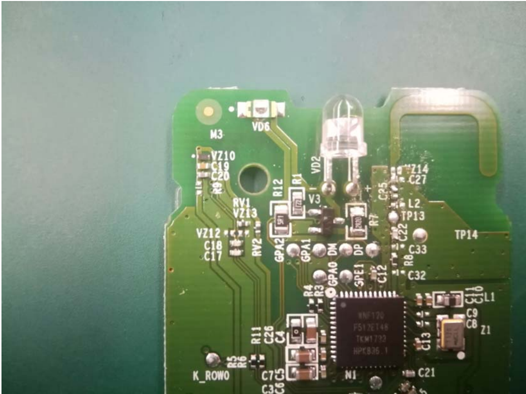
FIGURE 7 TV REMOTE CONTROL (M/N: ERF3A69) ANTENNA
