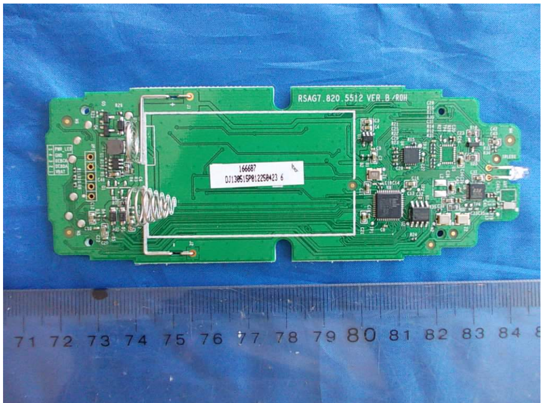
FIGURE 6 PULSE REMOTE CONTROL (M/N: ERF6B11) MAIN BOARD (BACK VIEW)
