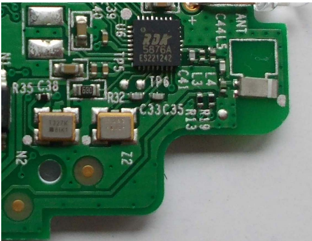
FIGURE 8 PULSE REMOTE CONTROL (M/N: ERF6B11) RF PART ON MAIN BOARD
