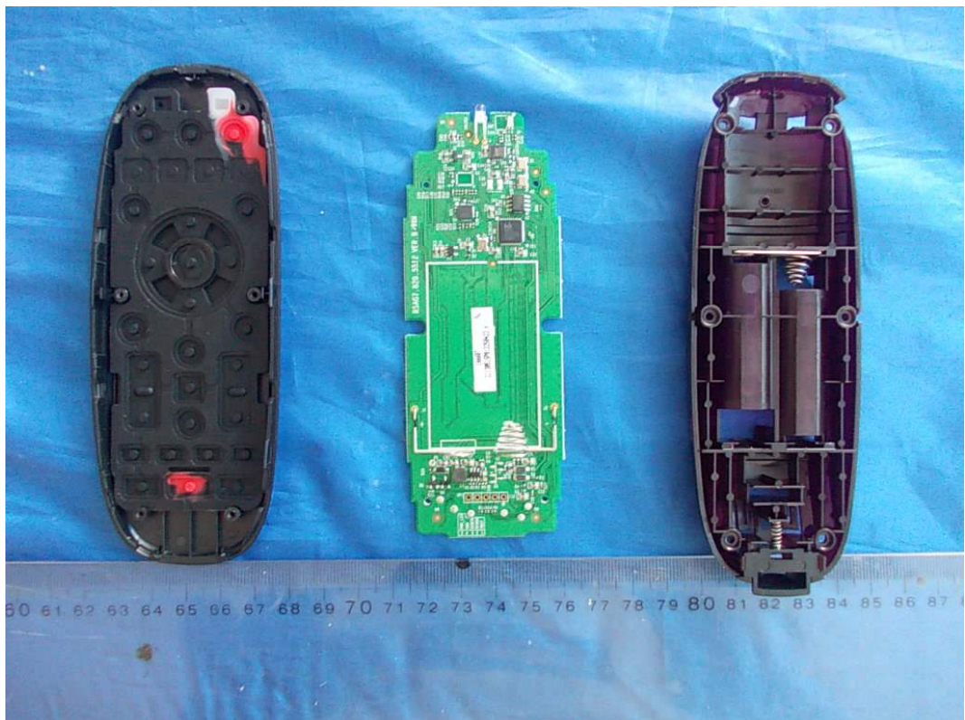
FIGURE 4 PULSE REMOTE CONTROL (M/N: ERF6B11) COVER REMOVED
