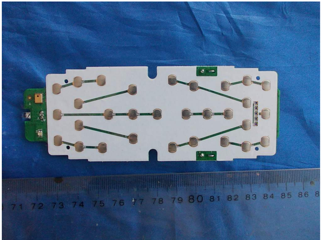
FIGURE 5 PULSE REMOTE CONTROL (M/N: ERF6B11) MAIN BOARD (FRONT VIEW)
