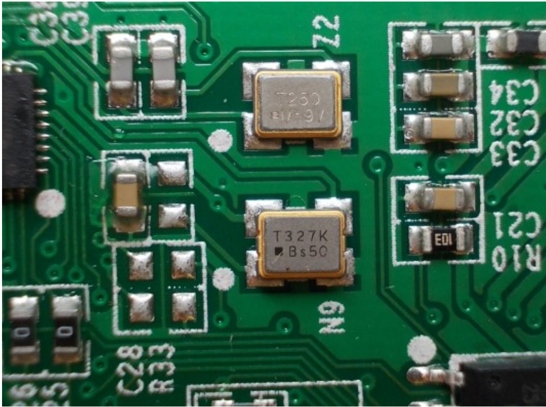
FIGURE 11 HISENSE PULSE WITH GOOGLE TV REMOTE CONTROL (M/N: ERF6B10) CRYSTAL #2 & #3 ON MAIN BOARD
