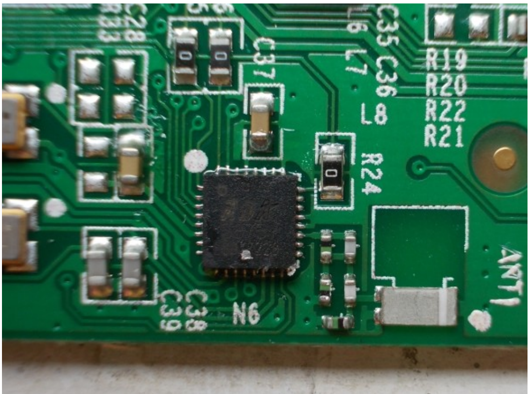
FIGURE 12 HISENSE PULSE WITH GOOGLE TV REMOTE CONTROL (M/N: ERF6B10) RF PART ON MAIN BOARD
