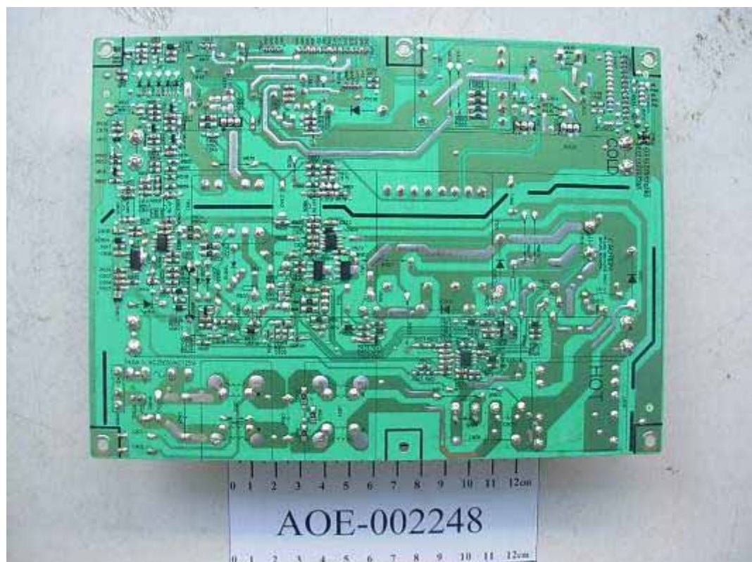
FIGURE 3 LCD TV (M/N: 37LC30S60) POWER BOARD (SOLDERED SIDE)
