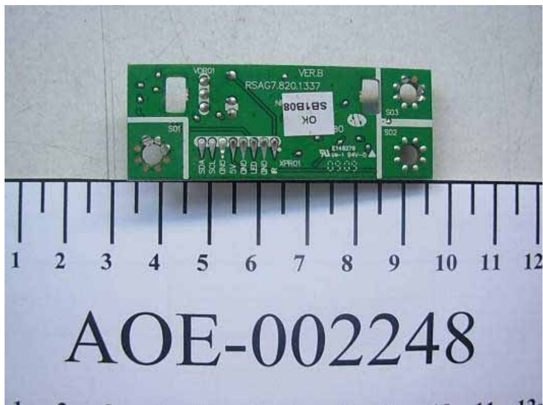
FIGURE 14 LCD TV (M/N: 37LC30S60) LED BOARD (SOLDERED SIDE)
