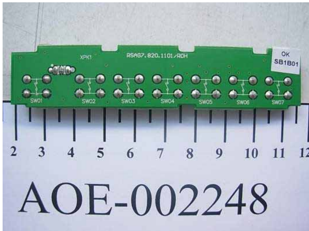
FIGURE 12 LCD TV (M/N: 37LC30S60) BUTTON BOARD (SOLDERED SIDE)
