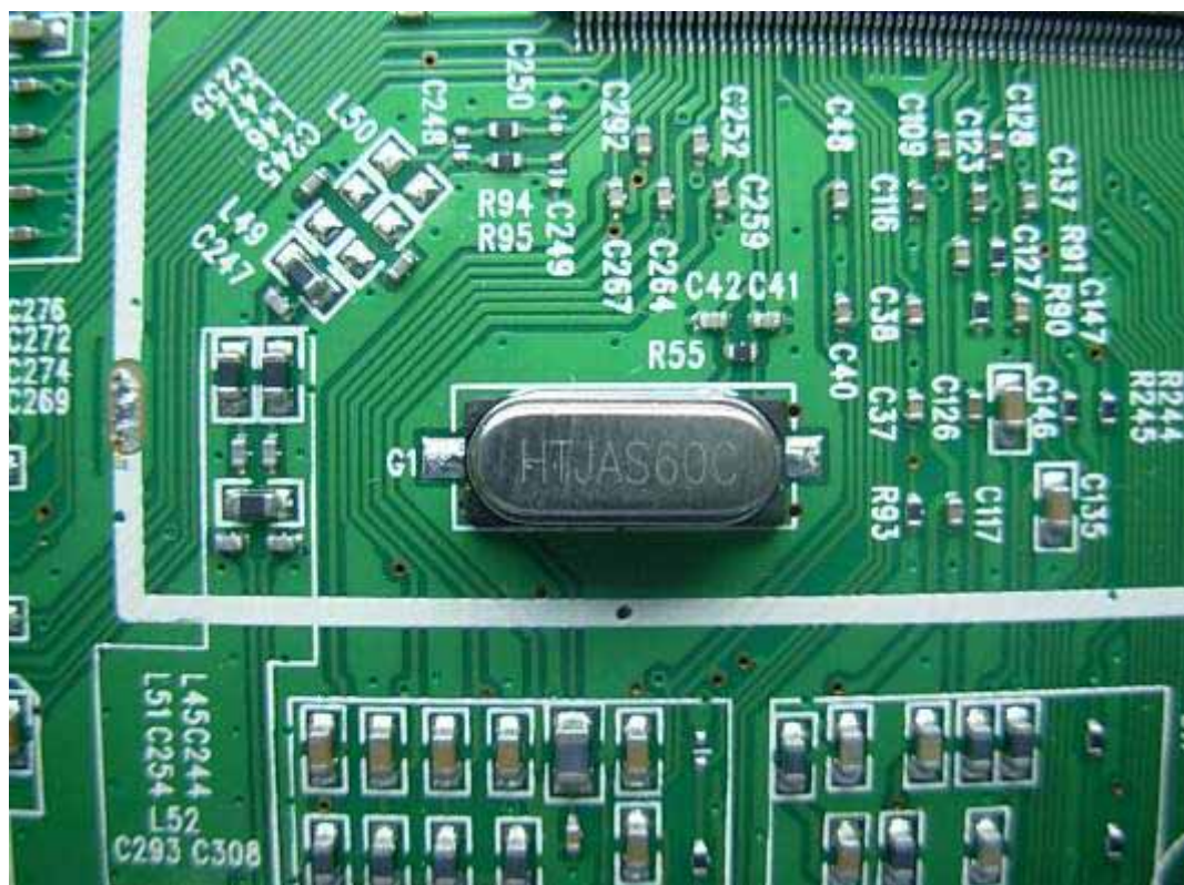
FIGURE 7 LCD TV (M/N: 37LC30S60) CRYSTAL
