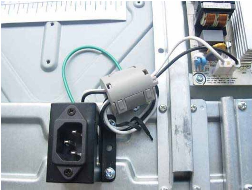
FIGURE 15 LCD TV (M/N: 37LC30S60) DEBUG 1
