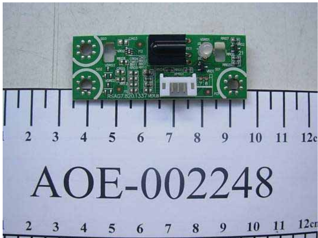
FIGURE 13 LCD TV (M/N: 37LC30S60) LED BOARD (COMPONENT SIDE)
