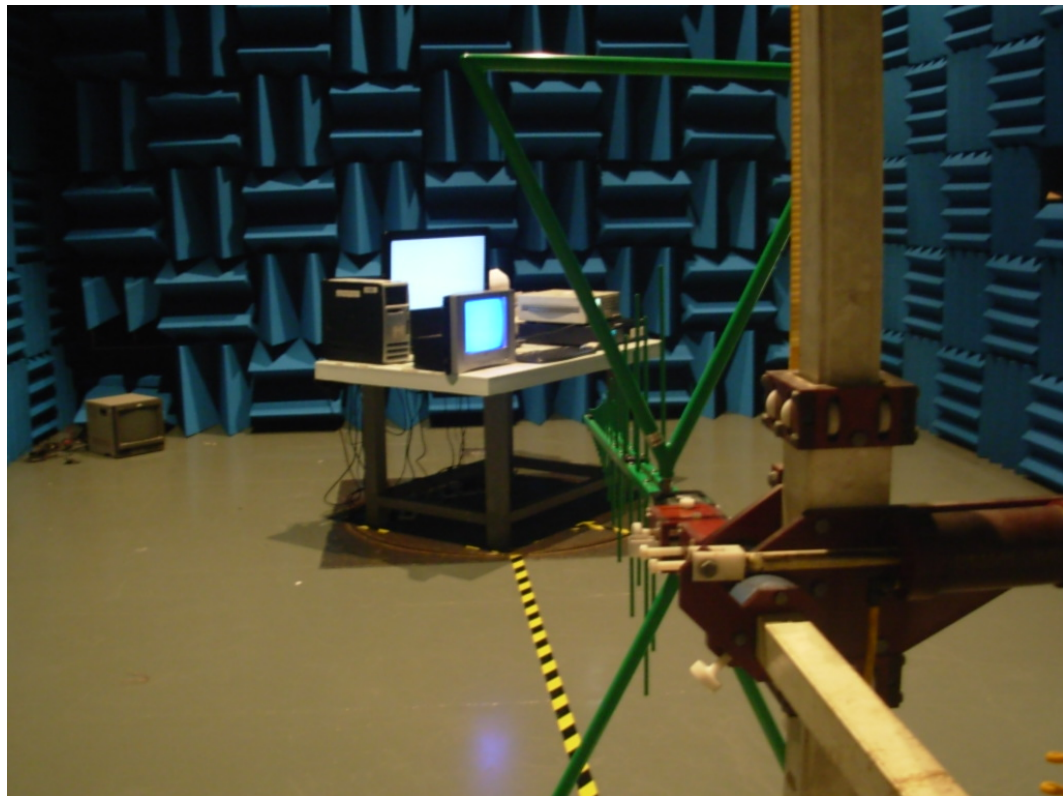
SETUP WITH MAXIMUM DETECTED EMISSION AT VERTICAL POLARIZATION (USB PLAY)
