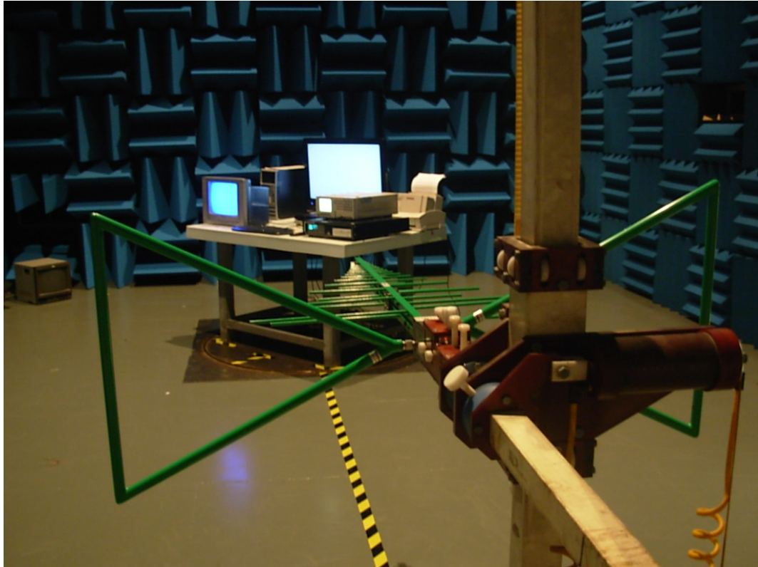
SETUP WITH MAXIMUM DETECTED EMISSION AT HORIZONTAL POLARIZATION (USB PLAY)
