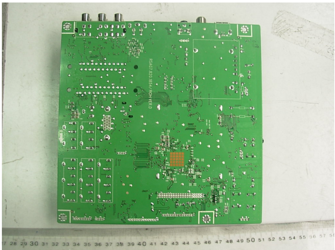
FIGURE 5 LCD TV (M/N: LCD32W57KCA) MAIN BOARD (SOLDERED SIDE)
