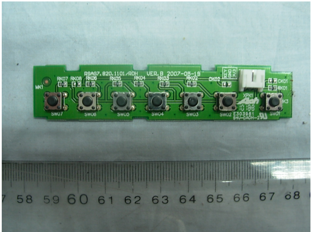
FIGURE 12 LCD TV (M/N: LCD32W57KCA) BUTTON BOARD (COMPONENT SIDE)
