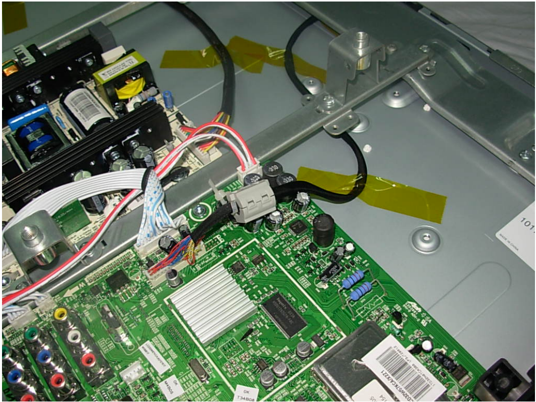
FIGURE 16 LCD TV (M/N: LCD32W57KCA) DEBUG 1
