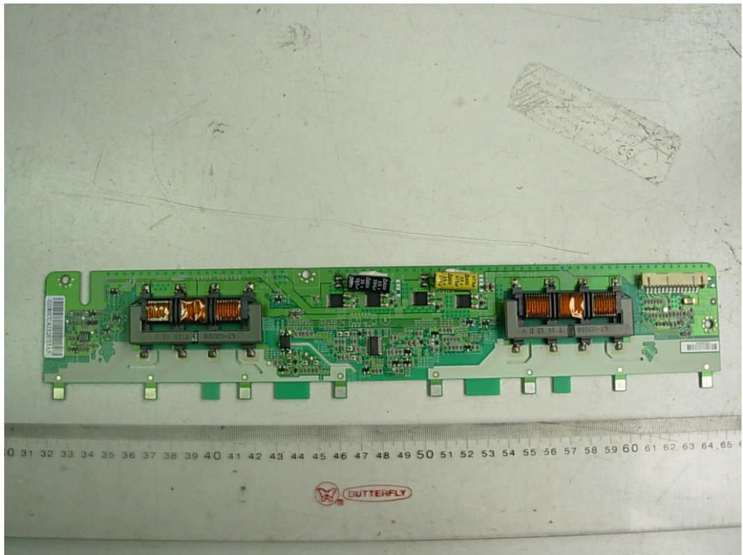
FIGURE 14 LCD TV (M/N: LCD32W57KCA) PANEL BOARD (COMPONENT SIDE)
