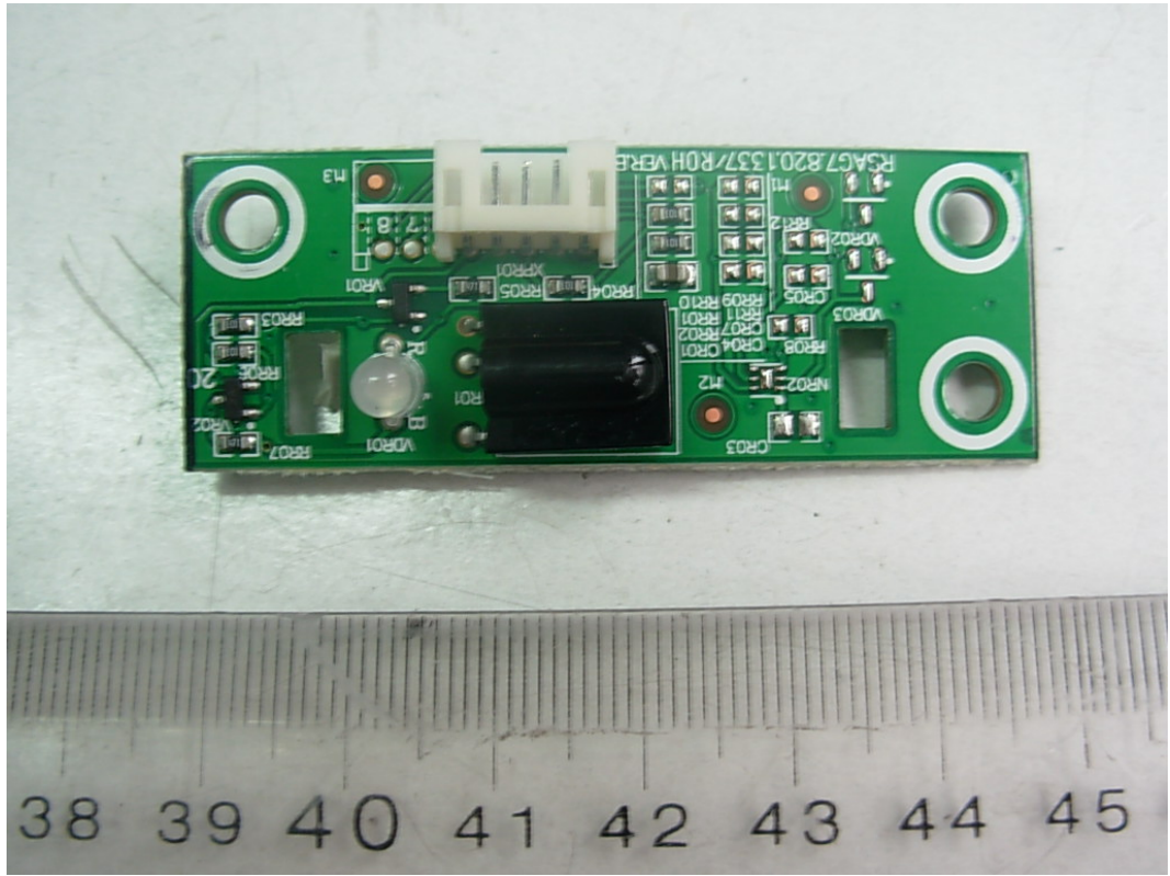
FIGURE 10 LCD TV (M/N: LCD32W57KCA) LED BOARD (COMPONENT SIDE)
