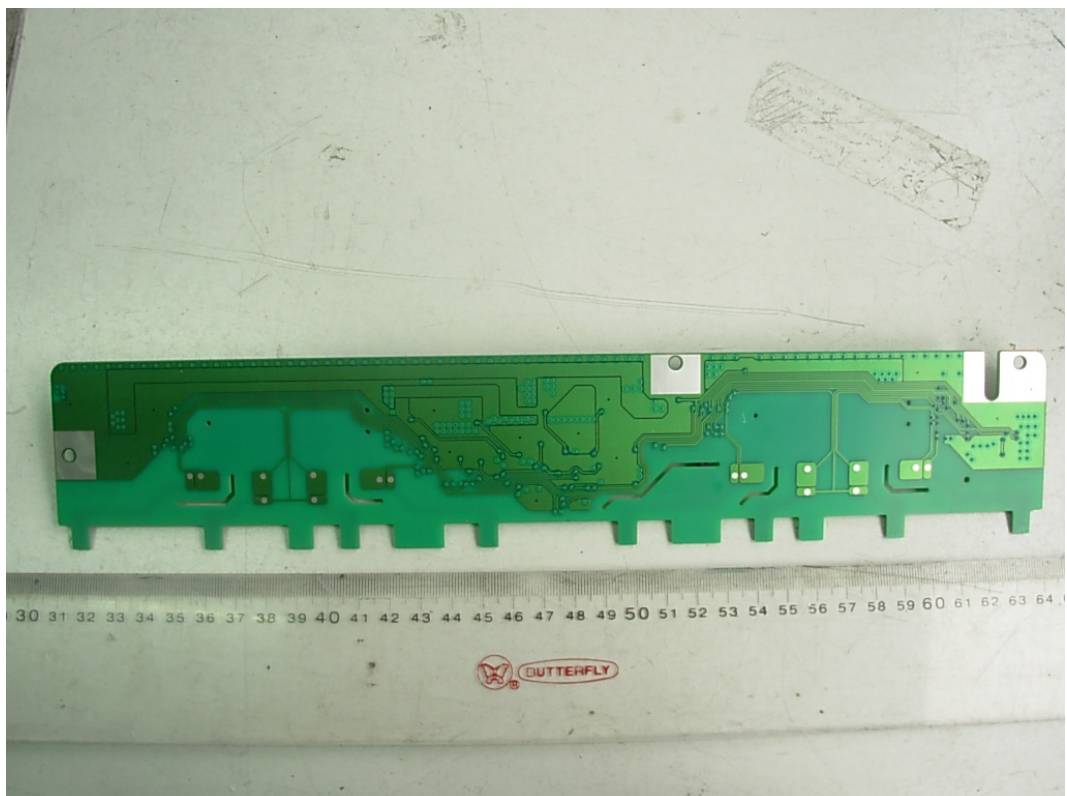
FIGURE 15 LCD TV (M/N: LCD32W57KCA) PANEL BOARD (SOLDERED SIDE)
