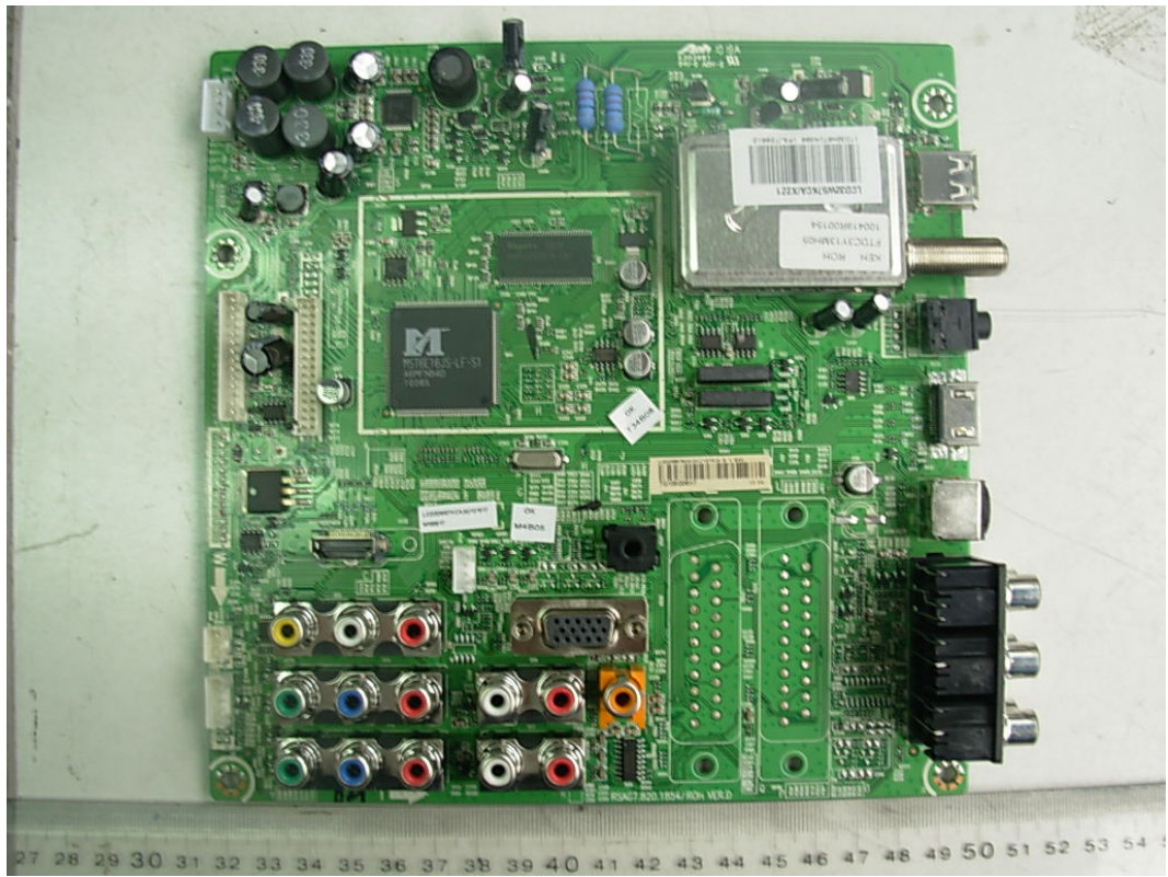
FIGURE 4 LCD TV (M/N: LCD32W57KCA) MAIN BOARD (COMPONENT SIDE)
