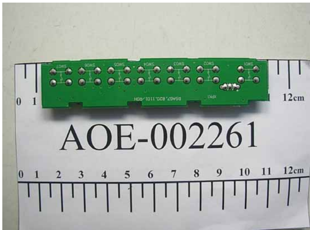
FIGURE 11 LCD TV (M/N: LHD32W57US) BUTTON BOARD (SOLDERED SIDE)
