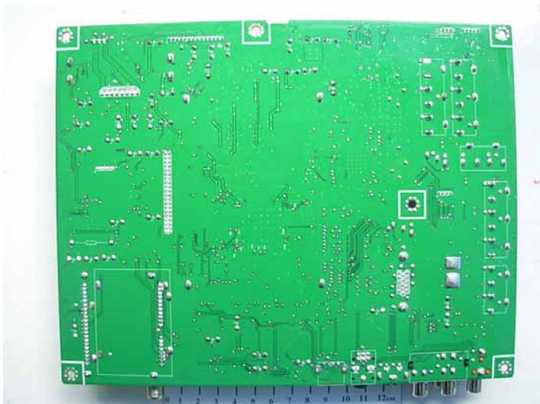
FIGURE 5 LCD TV (M/N: LHD32W57US) MAIN BOARD (SOLDERED SIDE)
