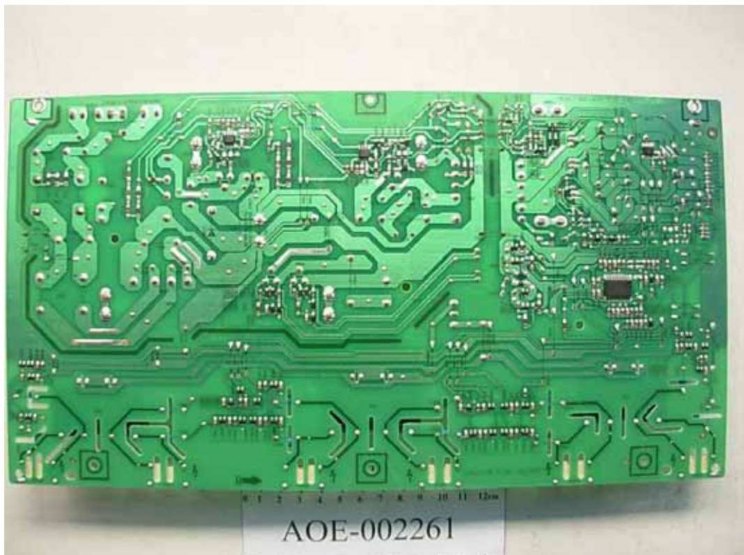
FIGURE 3 LCD TV (M/N: LHD32W57US) POWER BOARD (SOLDERED SIDE)
