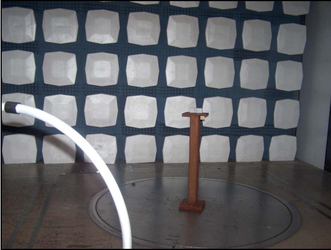
Photograph 1. Radiated Spurious
