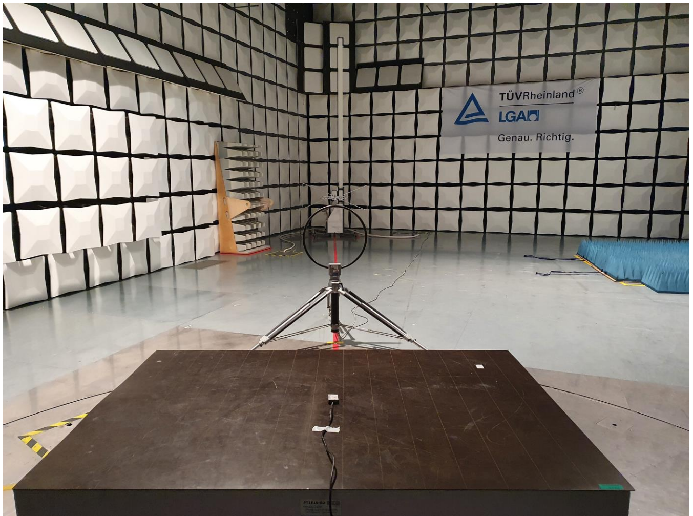
Bild / Picture 2: Test Setup, Radiated Measurements (9 kHz - 30 MHz)
