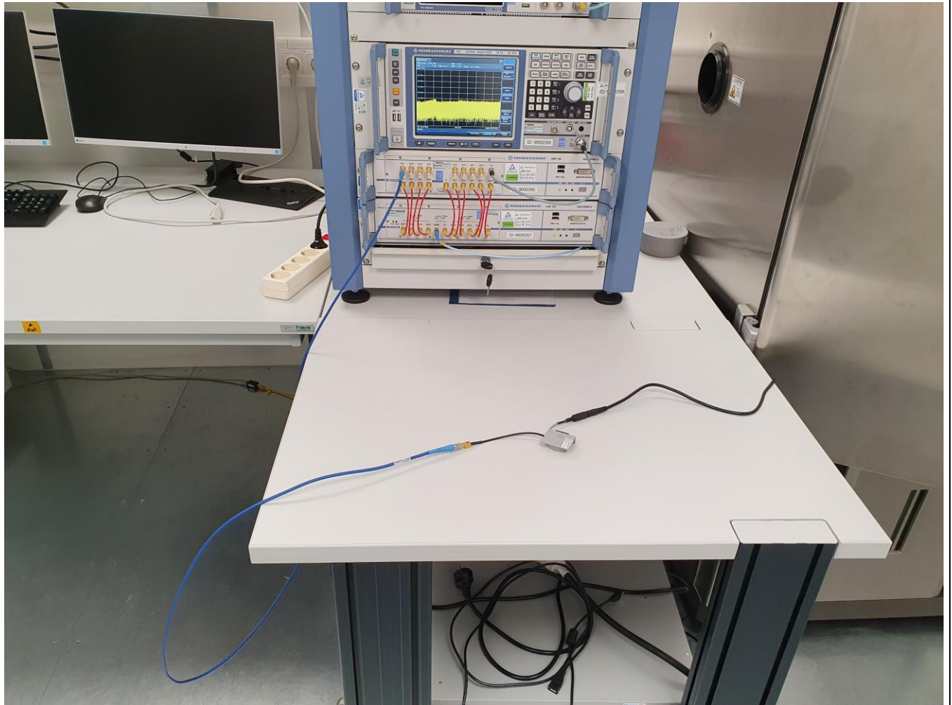
Bild / Picture 1: Test Setup, Conducted Measurements
