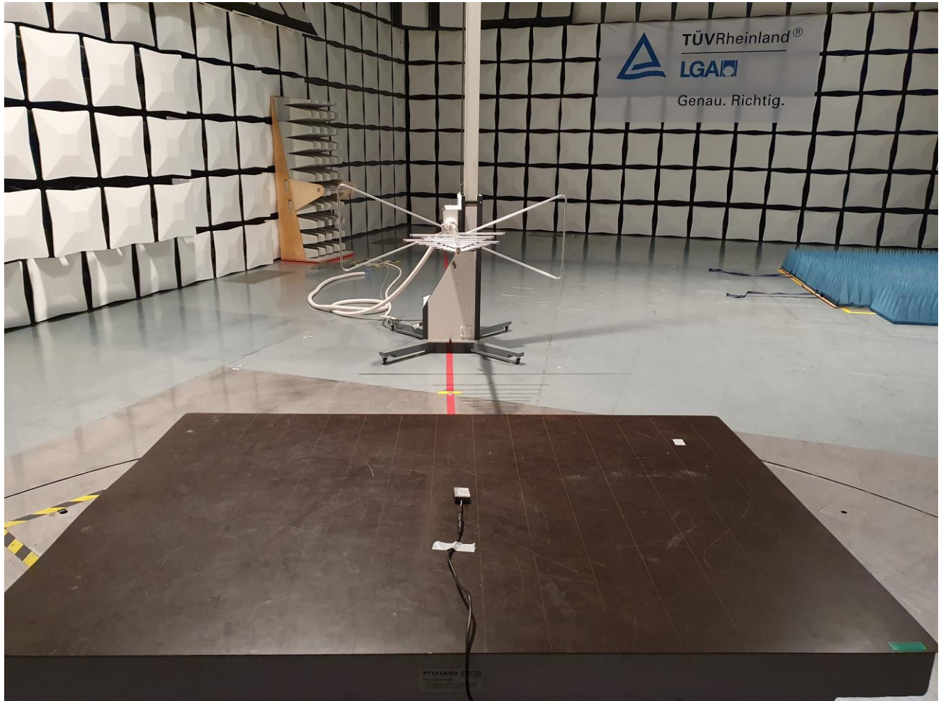
Bild / Picture 3: Test Setup, Radiated Measurements (30 MHz - 1 GHz)
