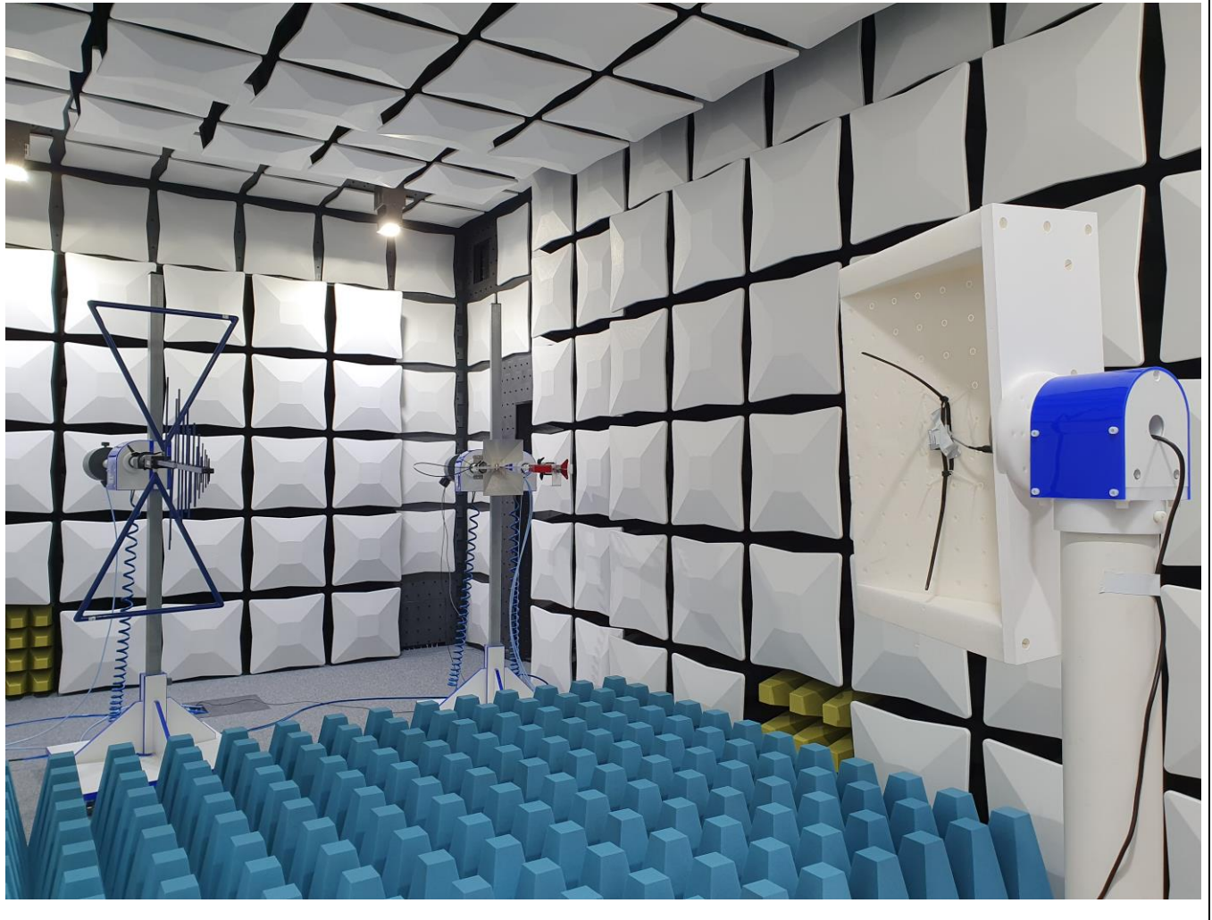
Bild / Picture 4: Test Setup, Radiated Measurements (1 GHz to 25 GHz)
