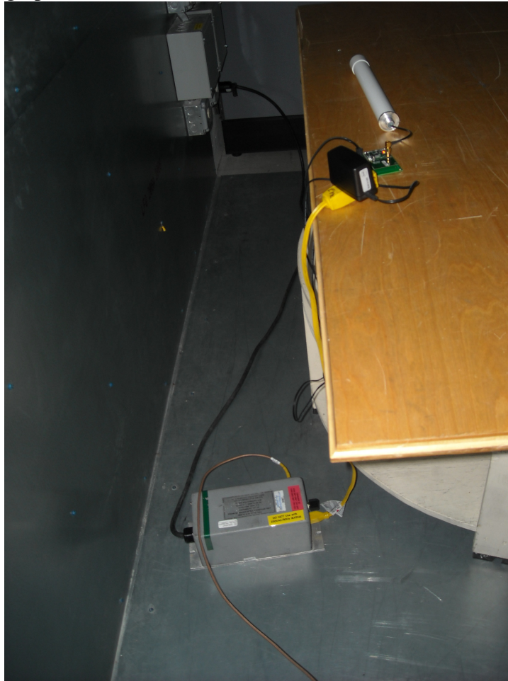
Line conducted emissions measurements – Rear
