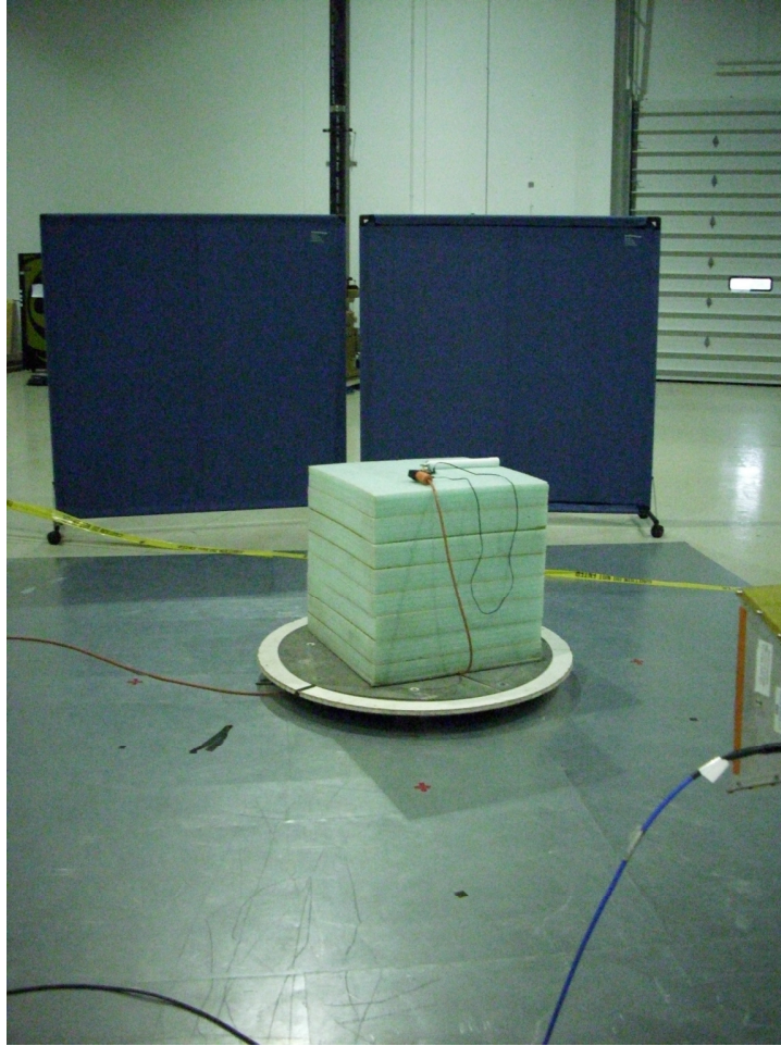
Radiated Measurements above 1GHz - OATS
