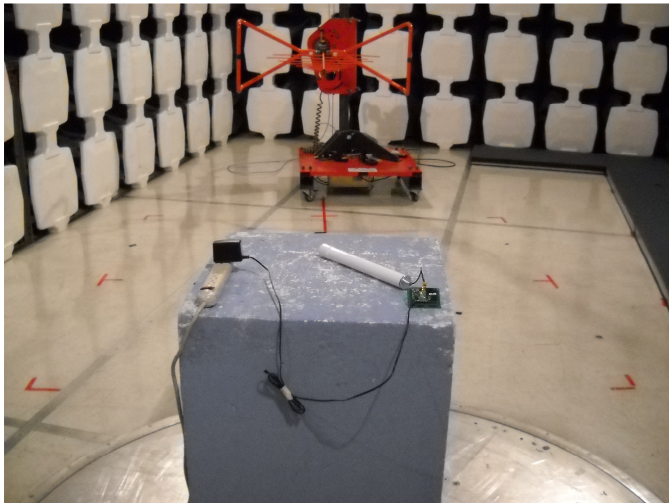
Radiated Measurements below 1GHz – Anechoic Chamber - Rear
