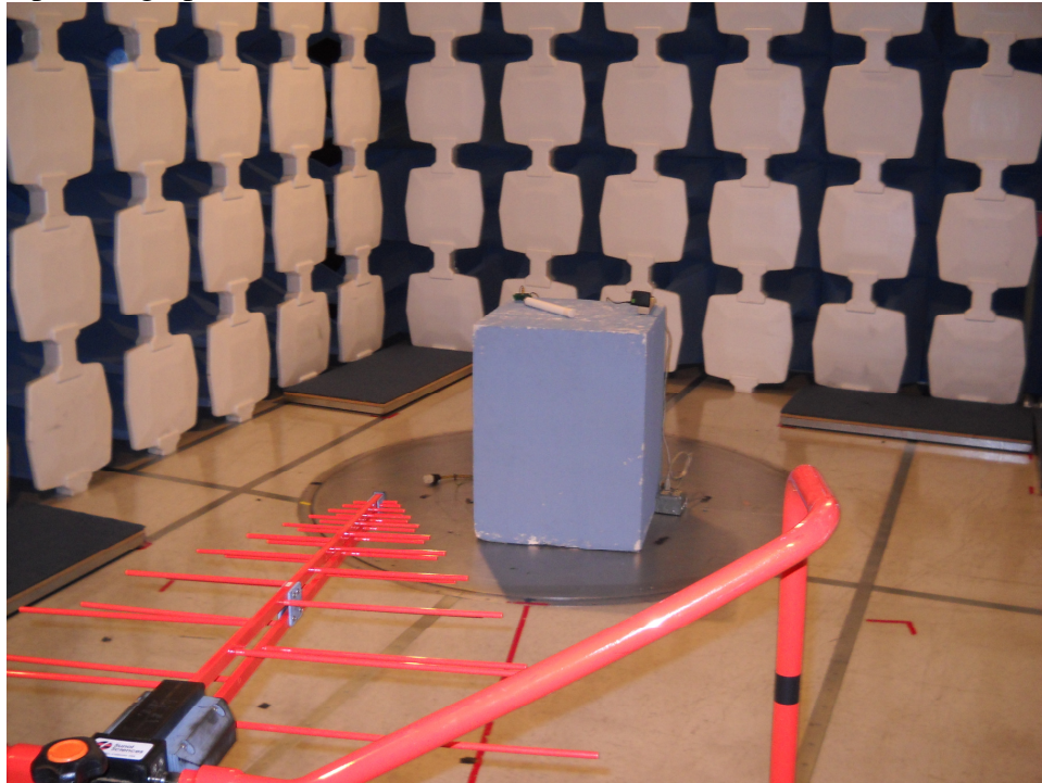
Radiated Measurements below 1GHz – Anechoic Chamber - Front
