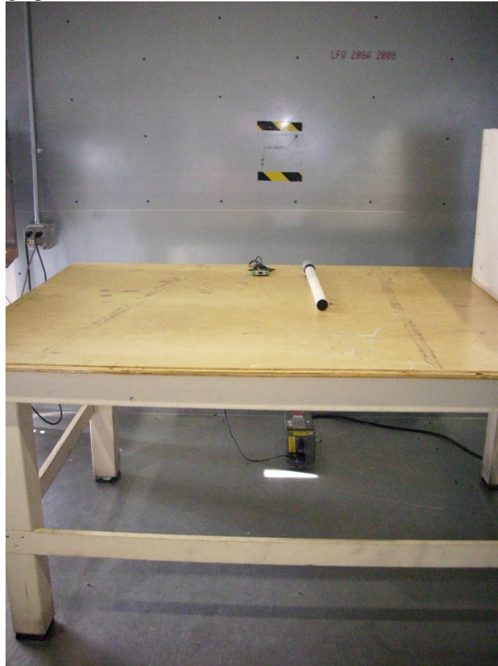
AC mains conducted emissions - Front
