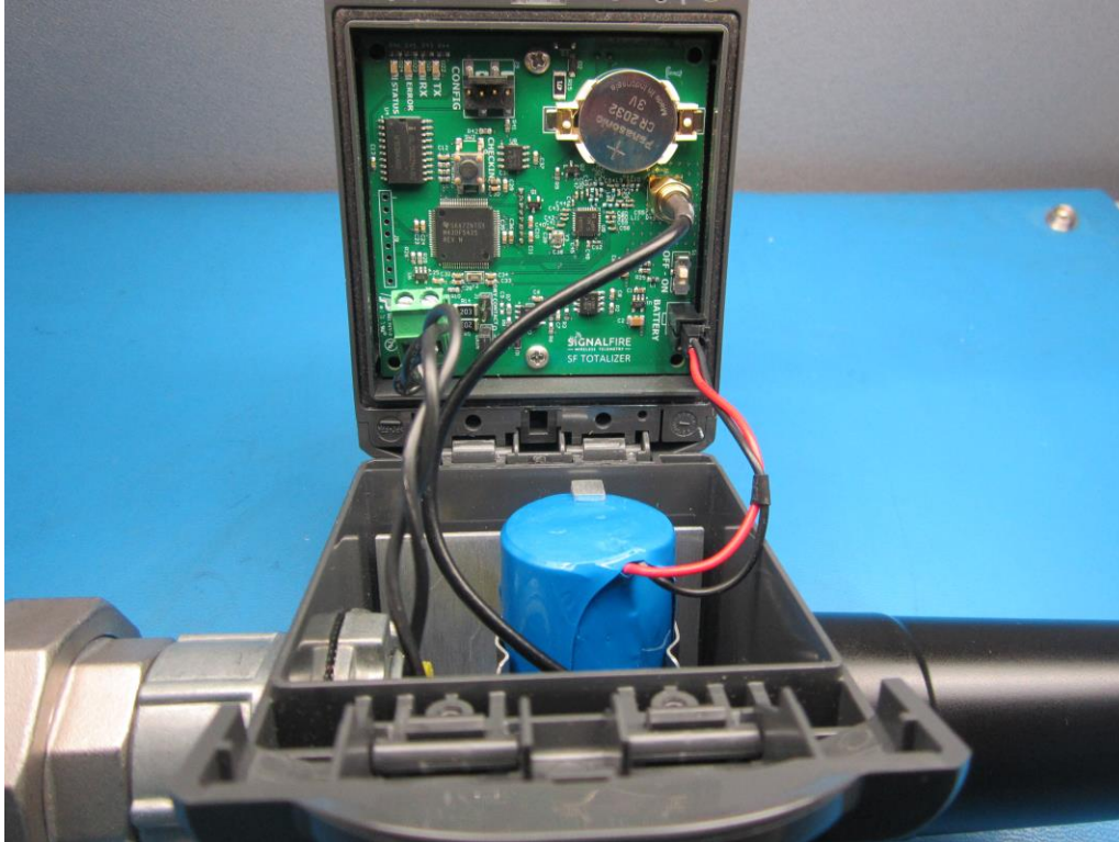
Signal Fire Telemetry, Internal connections
