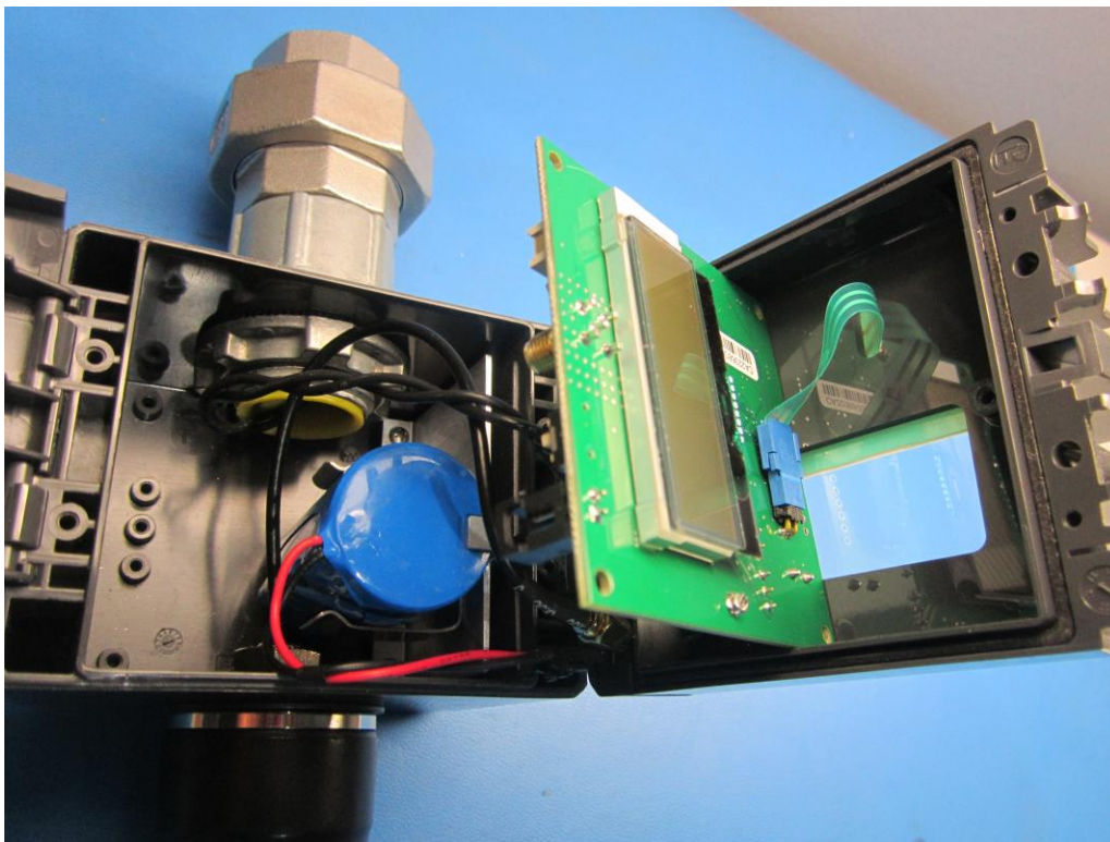
Signal Fire Telemetry, PCB connection to front control button
