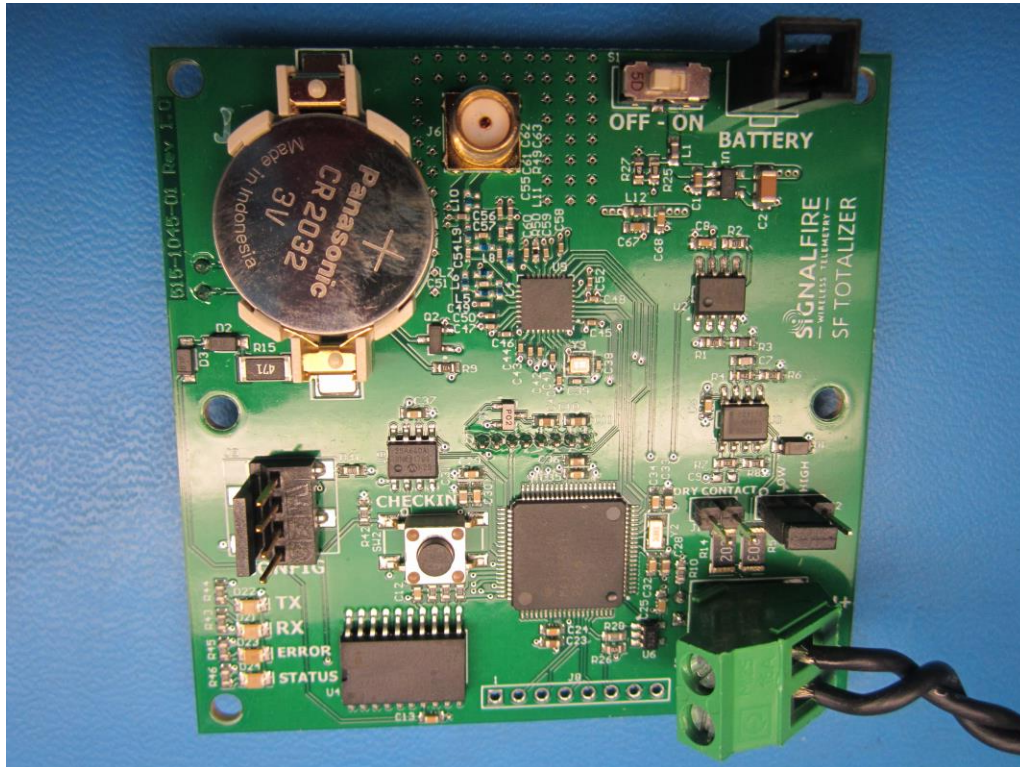
Signal Fire Telemetry, PCB, Bottom
