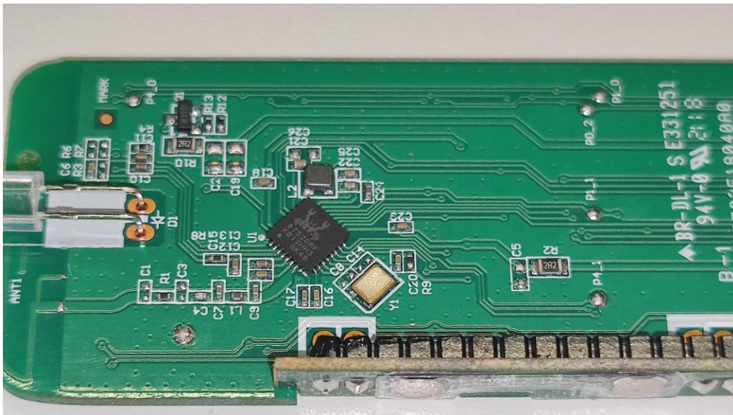
PCB with IC: RTL8752CRF
