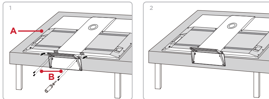
Screws M5x20mm
