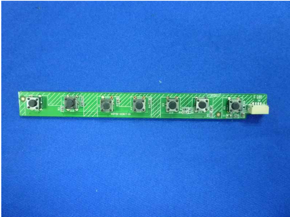
Figure 34 Frontside of the PCB
