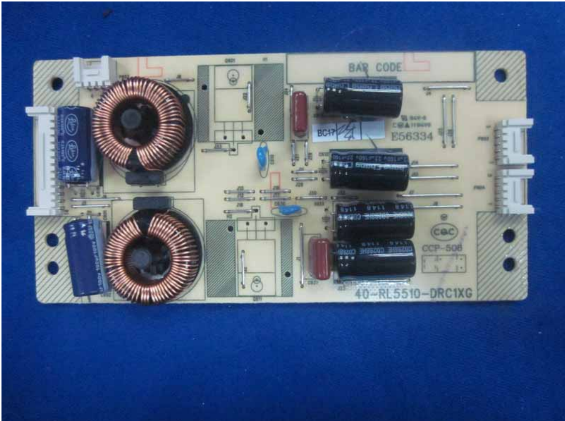
Figure 27 Frontside of the PCB
