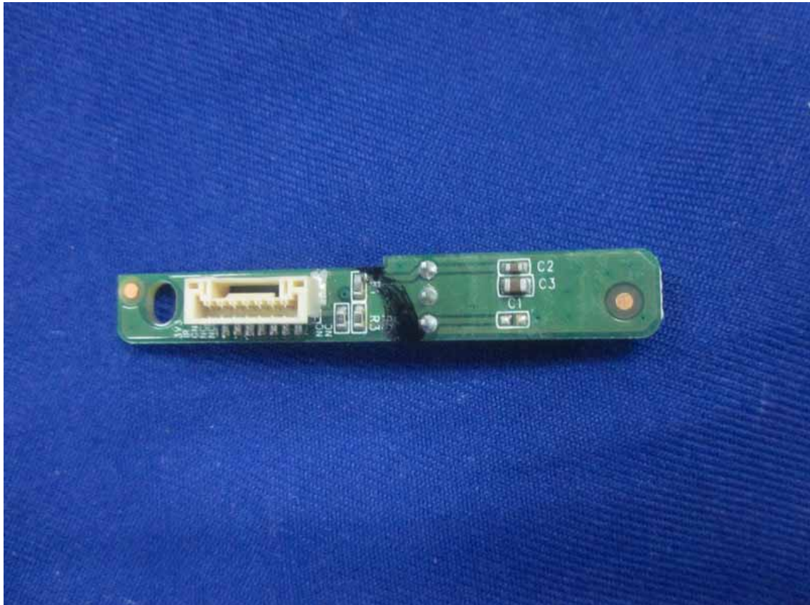
Figure 31 Frontside of the PCB
