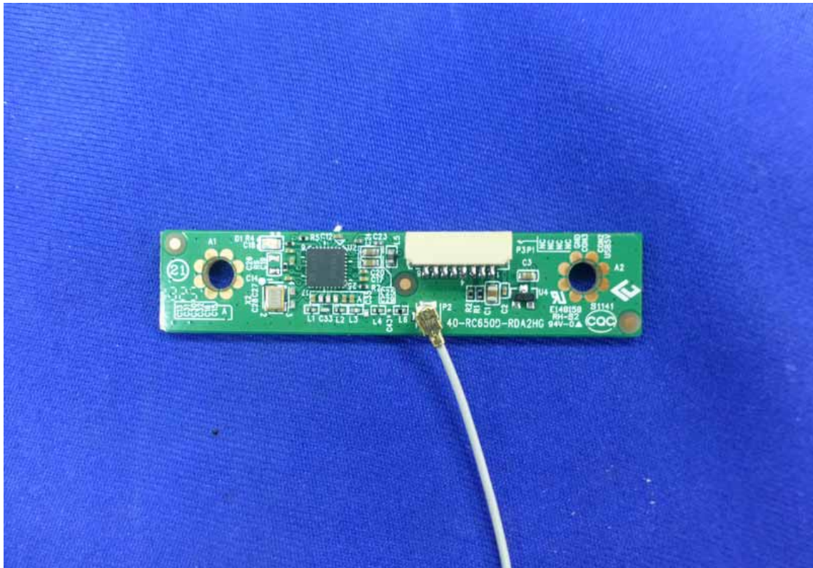
Figure 24 Frontside of the PCB Board
