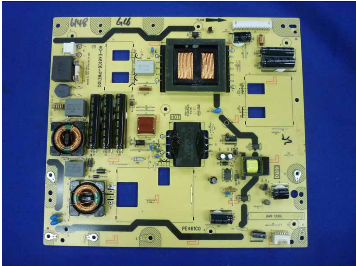
Figure 18 Frontside of the Power Board
