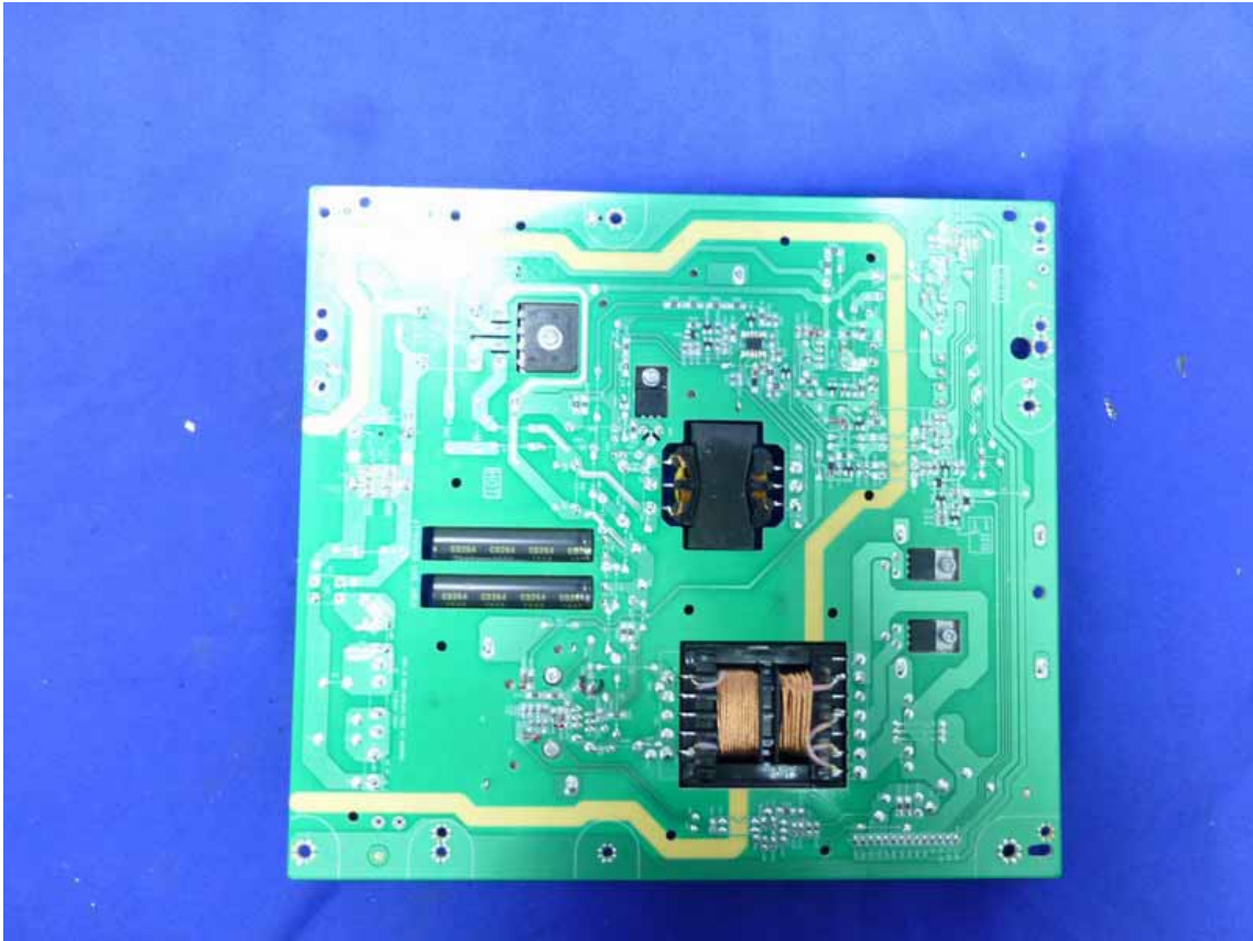
Figure 19 Backside of the Power Board
