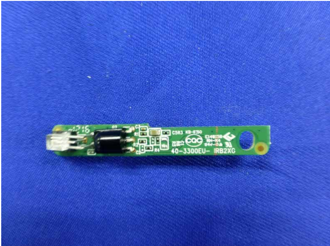
Figure 28 Backside of the PCB
