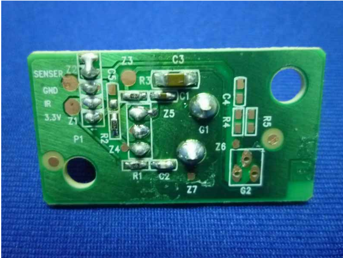
Figure 17 Frontside of the Control Board
