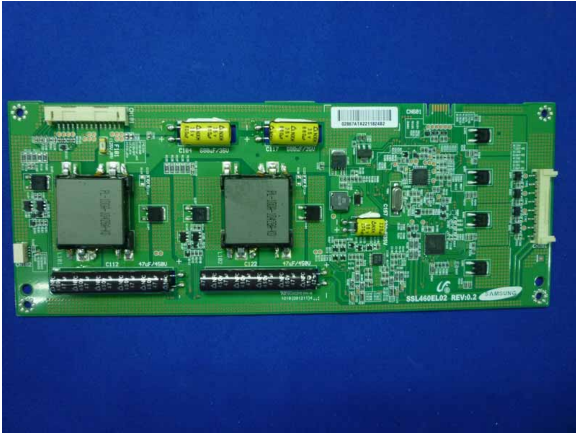
Figure 19 Frontside of the Inverter Board
