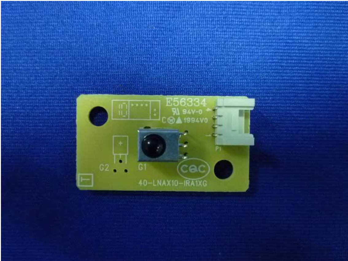
Figure 18 Backside of the Control Board
