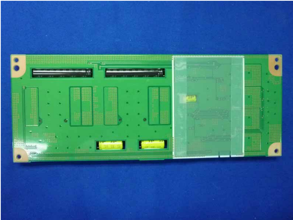
Figure 20 Backside of the Inverter Board
