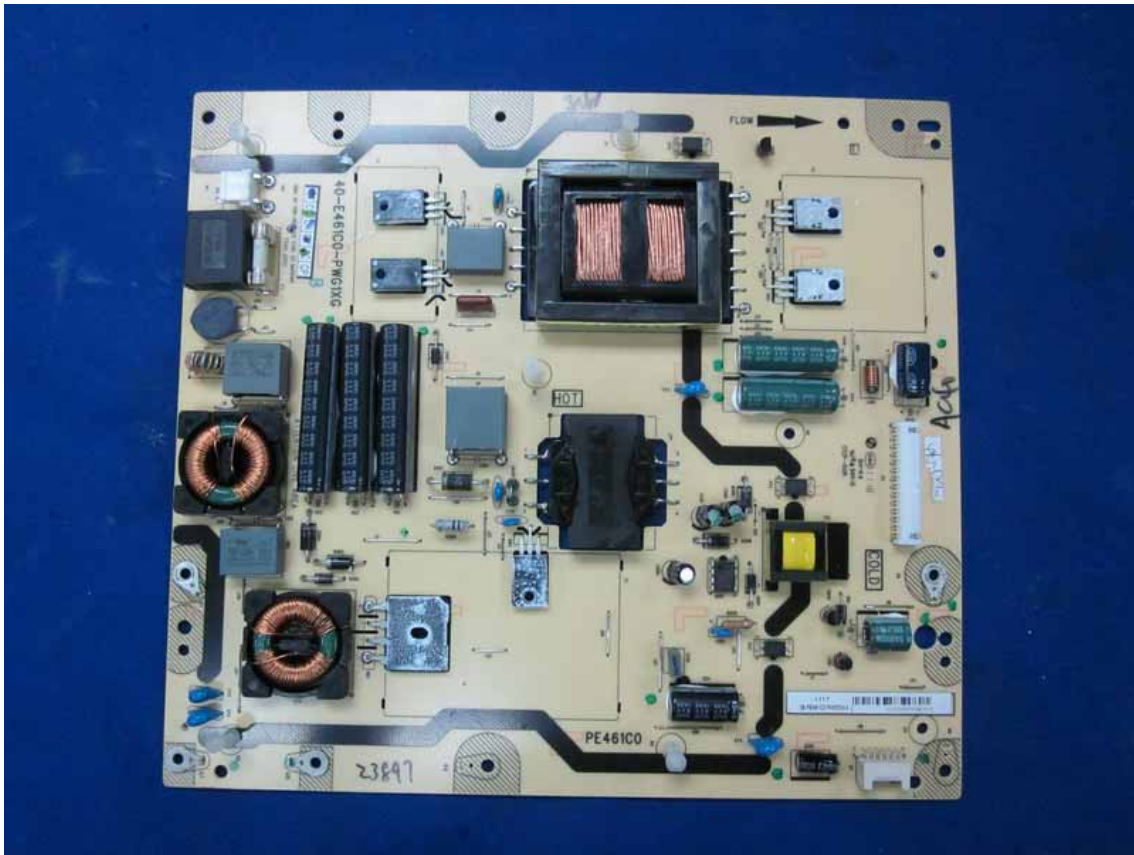
Frontside of the Power Board
