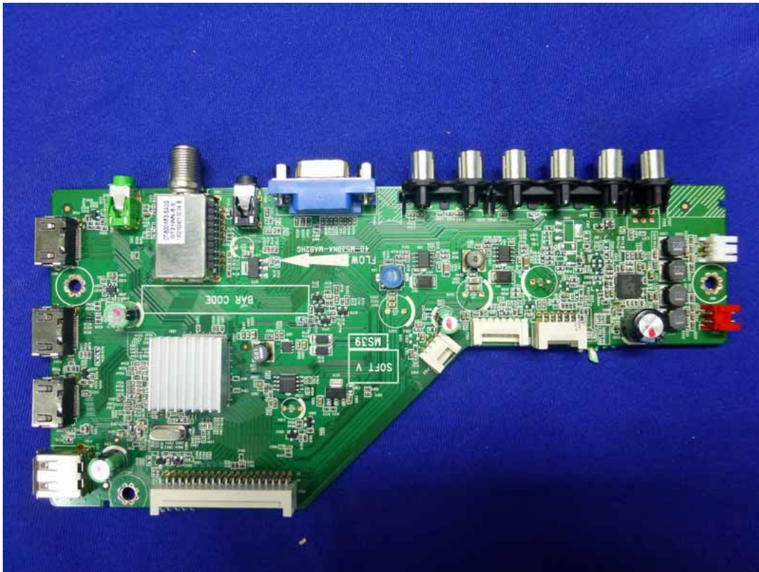
Figure 15 Frontside of the PCB
