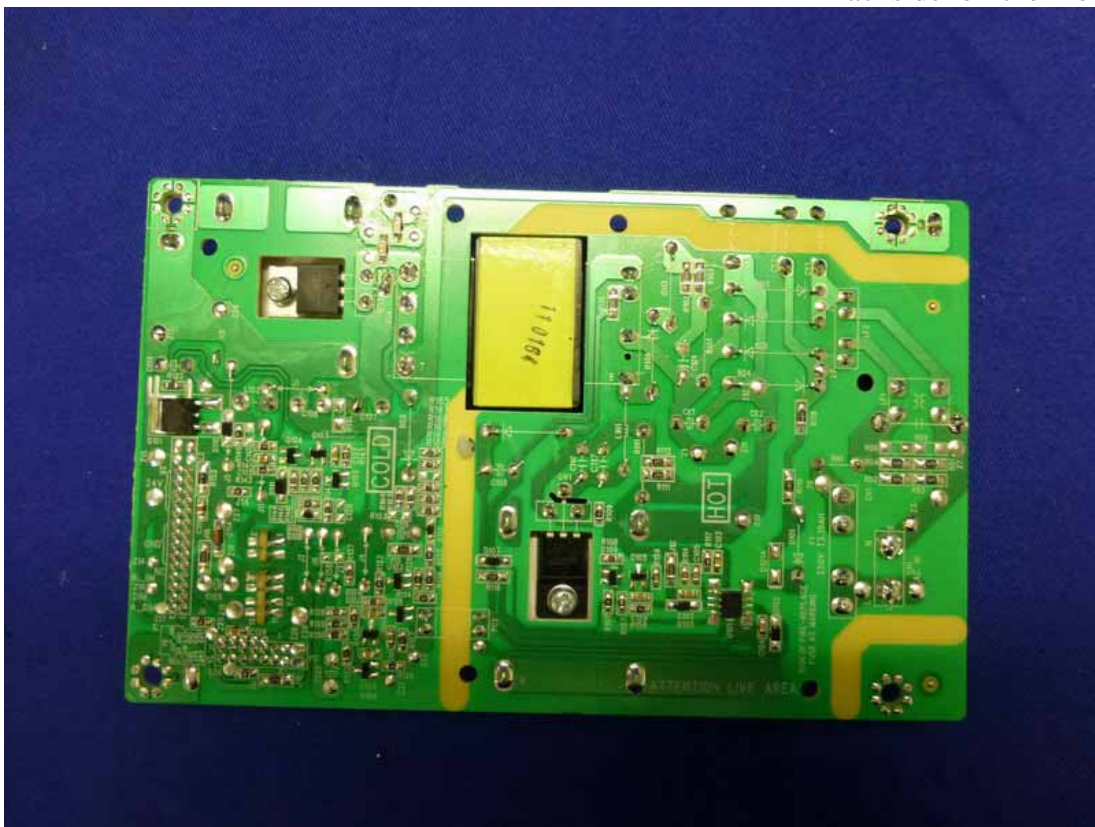
Backside of the Power Board
