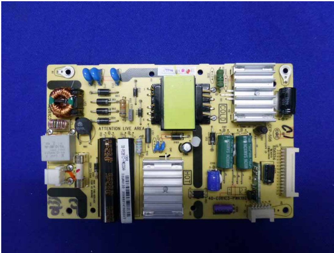
Frontside of the Power Board
