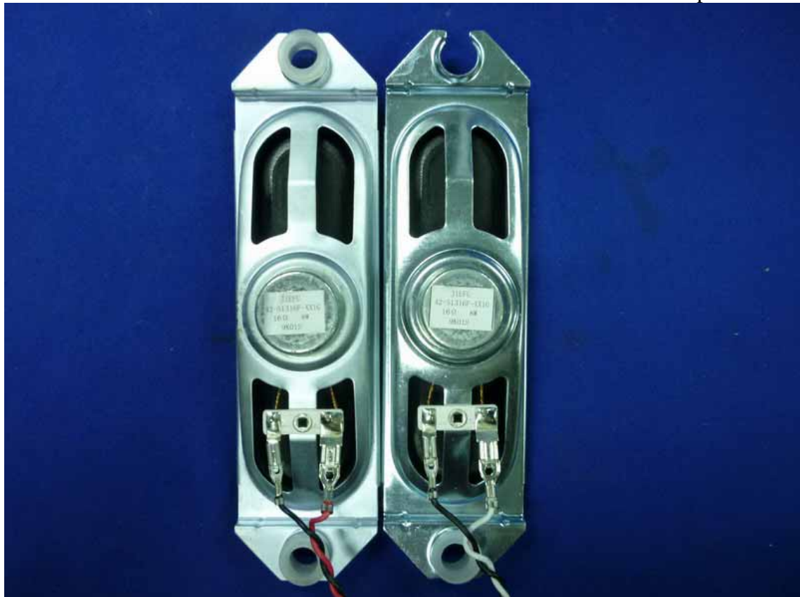
Figure 36 Speaker of the EUT
