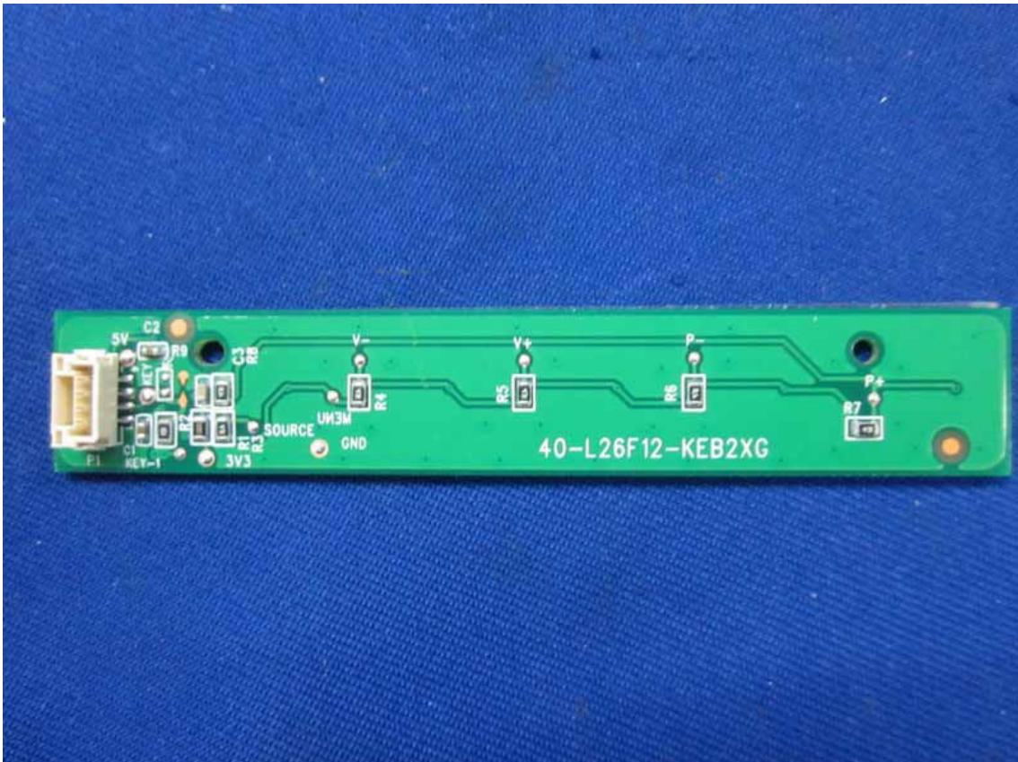
Figure 16 Backside of the Control Board
