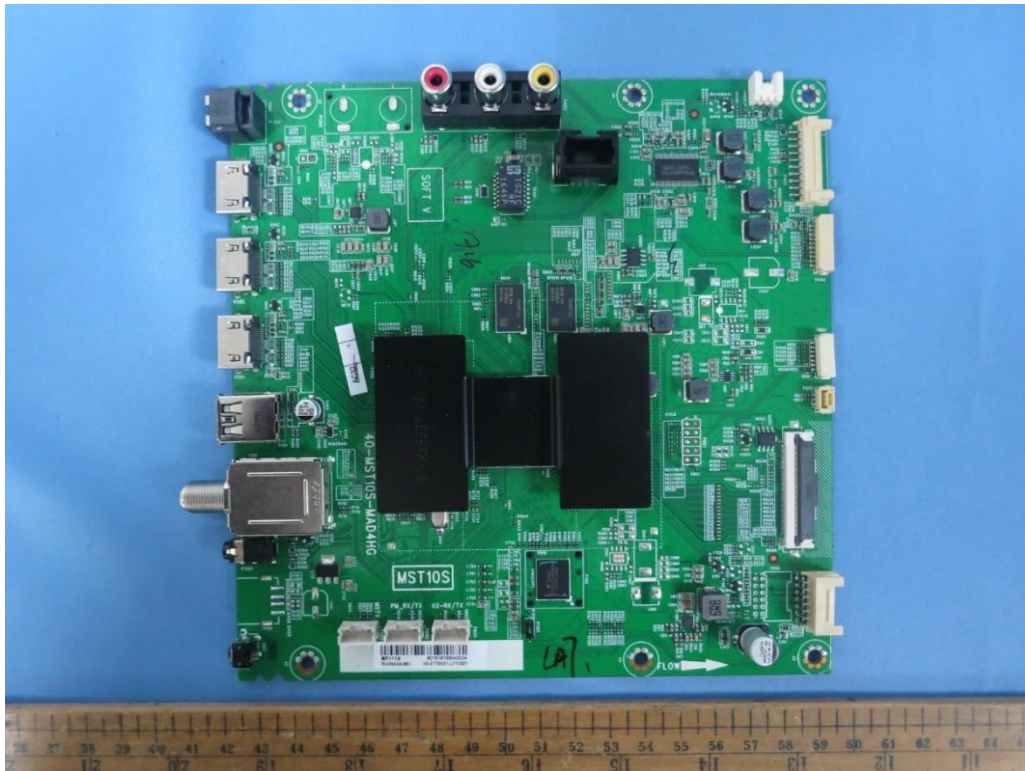
Mainboard(MST10S)
