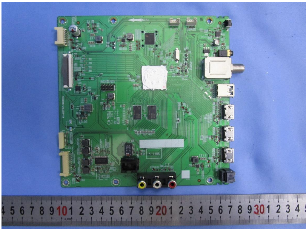
Mainboard(MST10C)
