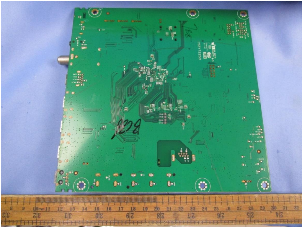
Mainboard(MST10S)
