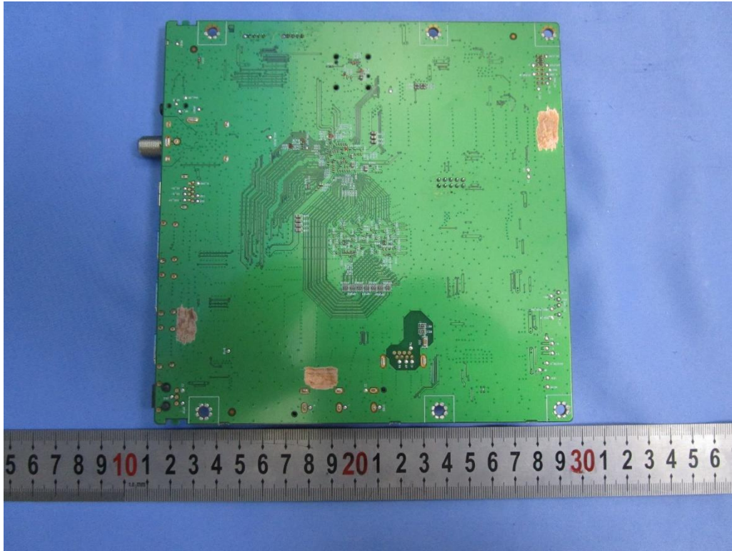
Mainboard(MST10C)
