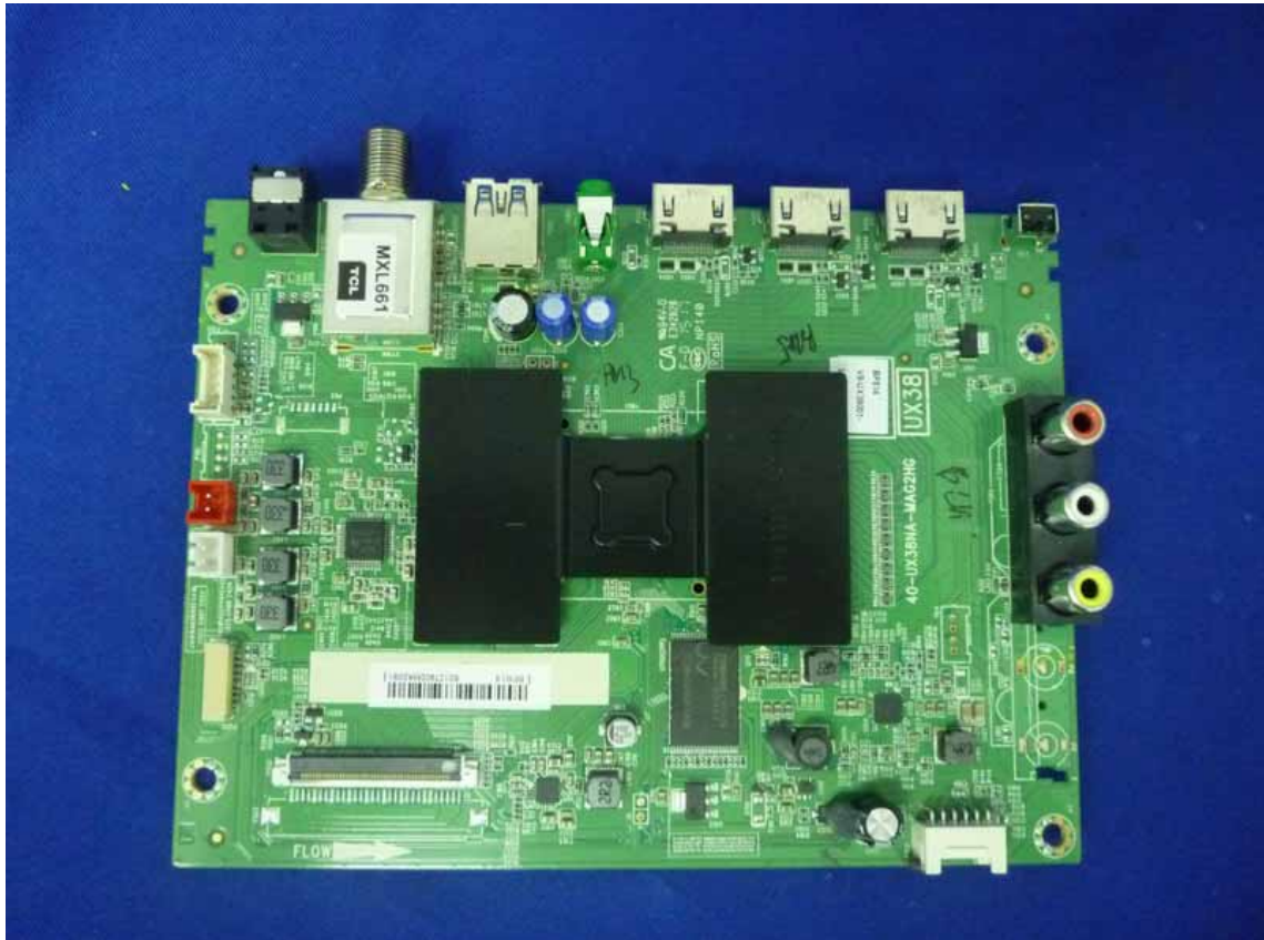
Figure 8 Frontside of the Main Board
