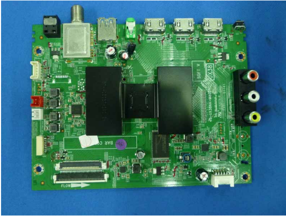
Figure 11 Frontside of the Main Board
