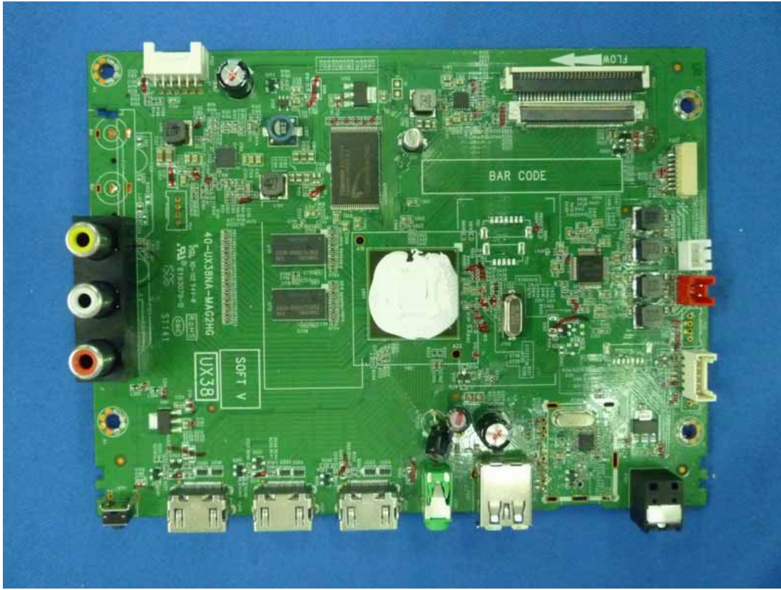
Figure 25 Frontside of the PCB Board
