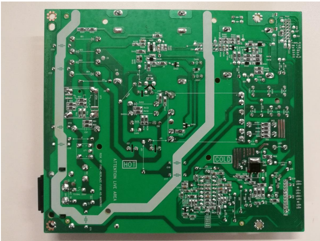
Power board Version 2
