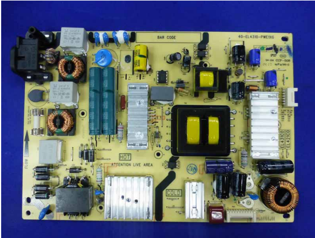
Figure 19 Frontside of the Power Board
