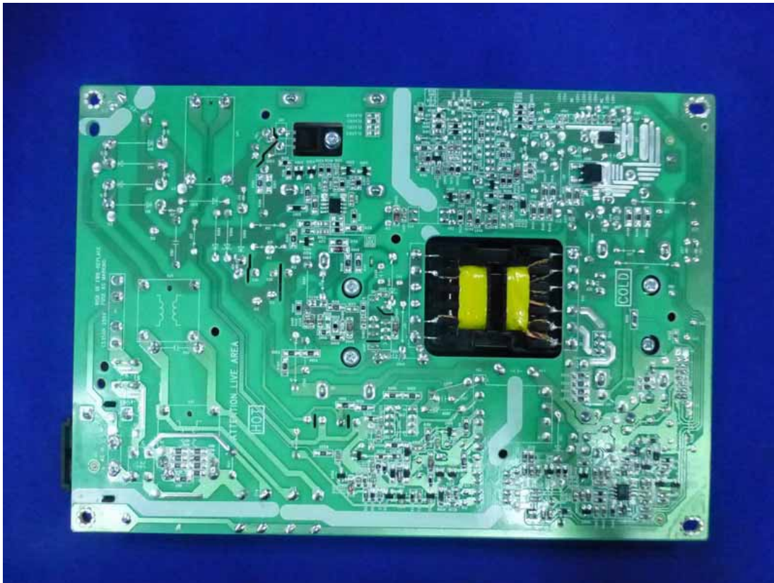
Figure 20 Backside of the Power Board
