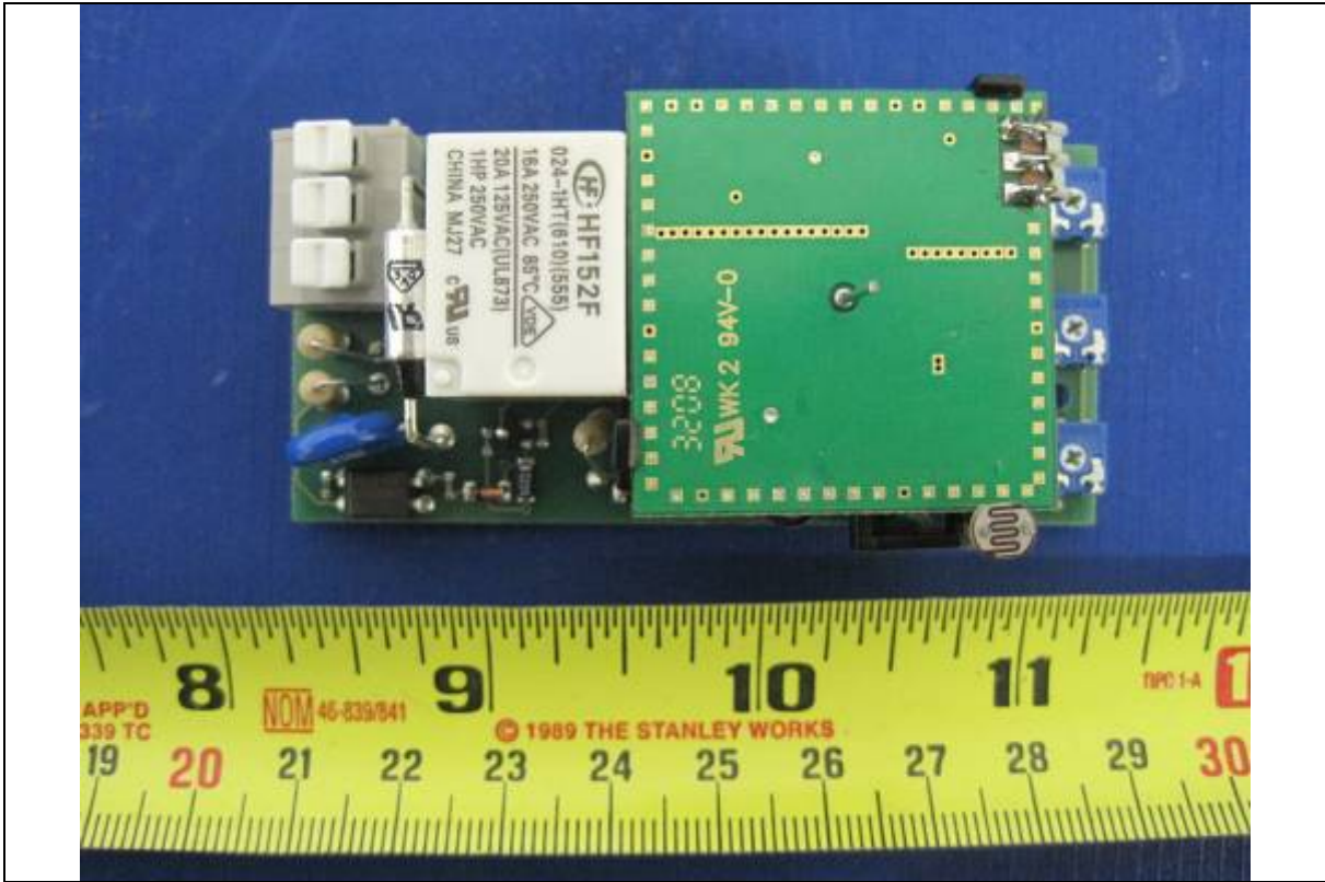
EUT Cover off View
