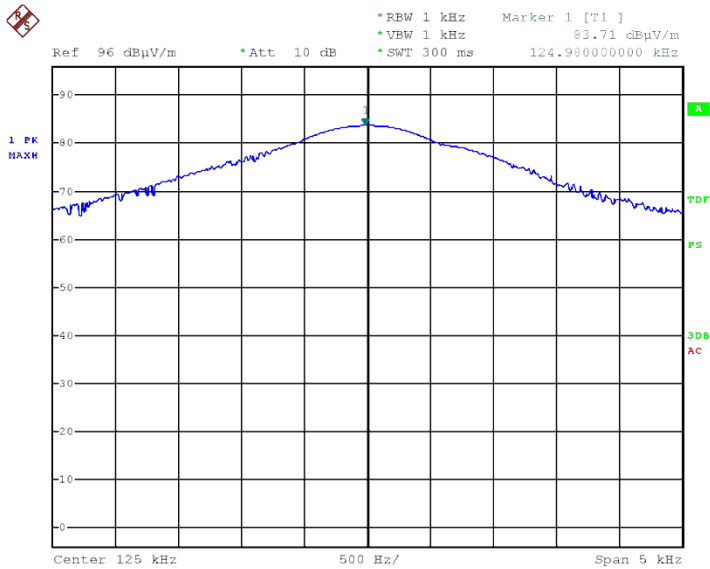
Figure 4. Field Strength of Fundamental, Low, Detector: Peak
