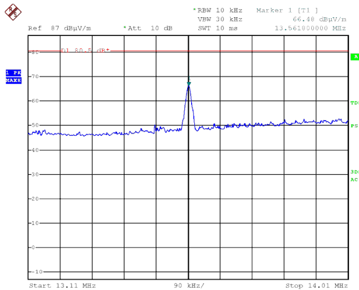
Figure 11. Field Strength of Fundamental, Horizontal
