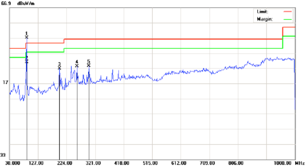
Test Result of Bottom Channel (88.1 MHz)
