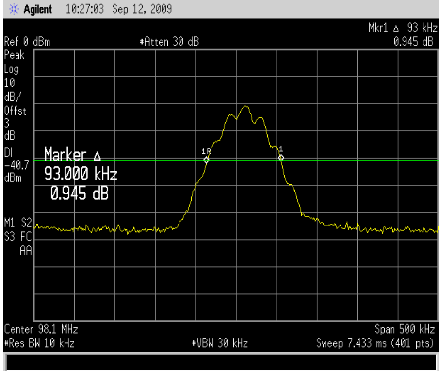
98.1MHZ bandwidth test plot
