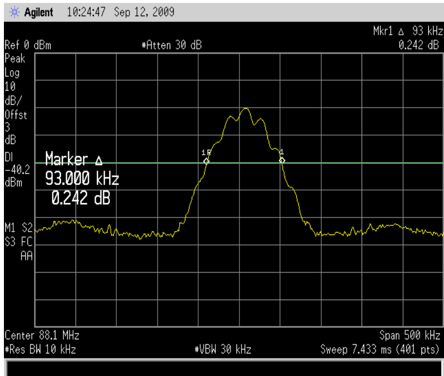
88.1MHZ bandwidth test plot
