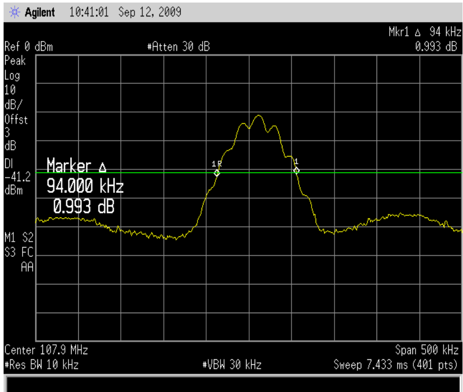
107.9MHZ bandwidth test plot
