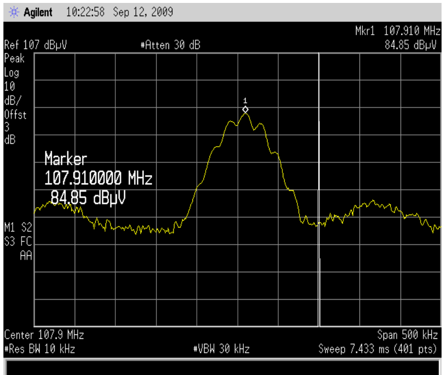
107.9MHZ Test Plot
