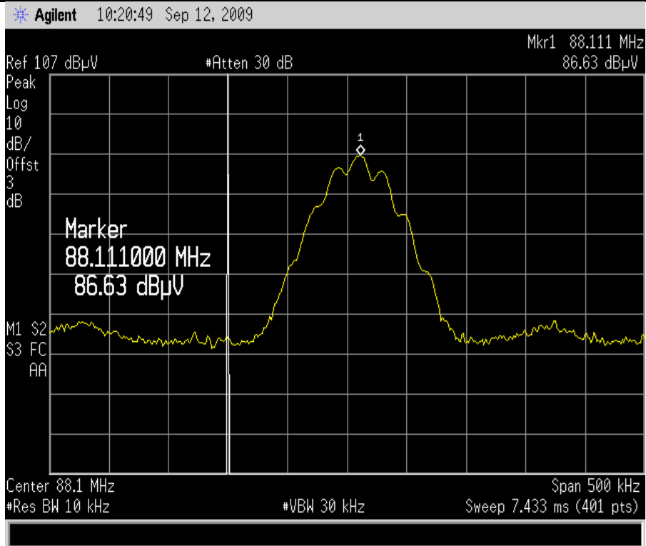
88.1MHZ Test Plot
