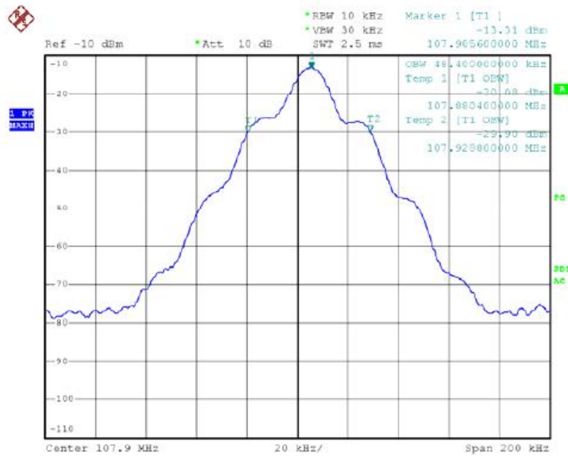
107.9MHz Test Plot
