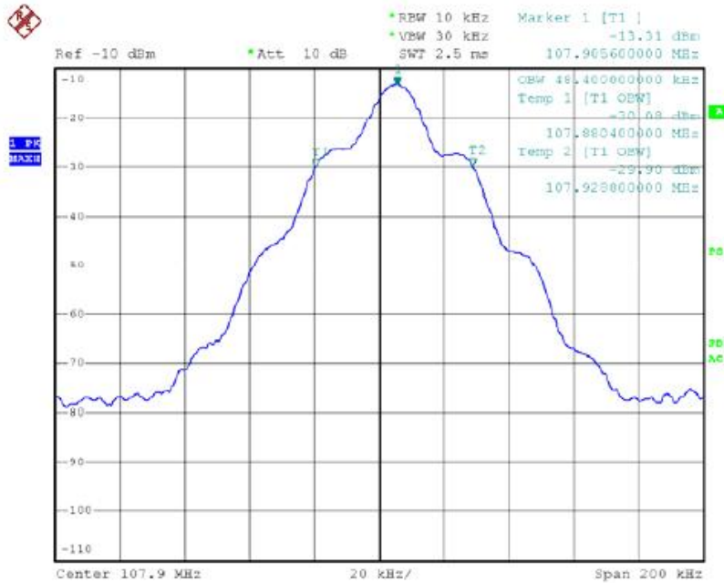
107.9MHz bandwidth test plot
