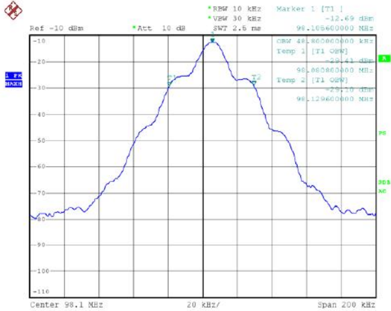
98.1MHz bandwidth test plot
