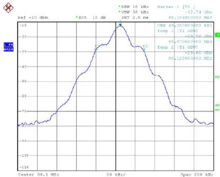
88.1MHZ bandwidth test plot
